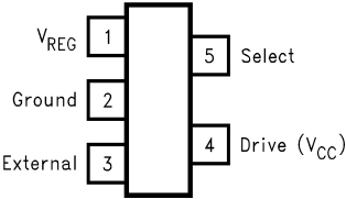
5-Lead SOT23-5 Surface Mount Package
