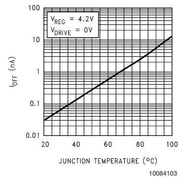
LM3620M5-4 Off State Current vs Temperature
