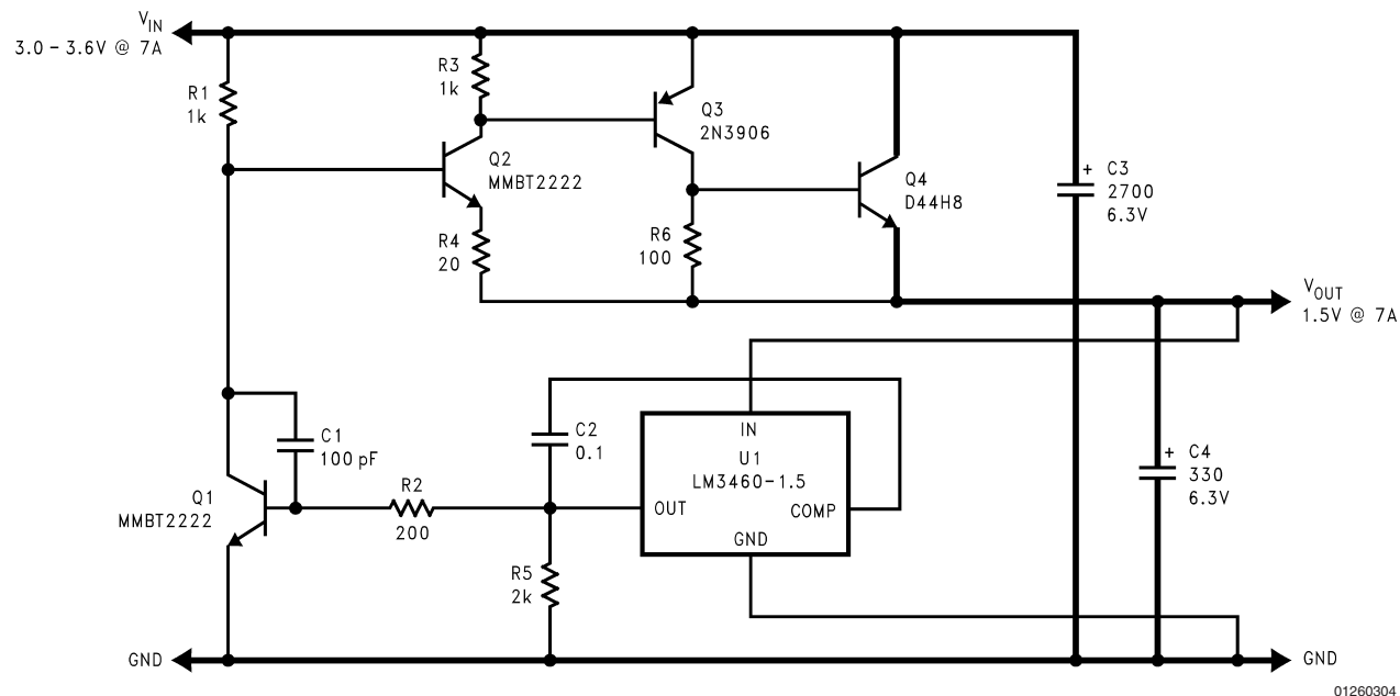
FIGURE 1. 1.5V Typical Application (See Application Information Section)
