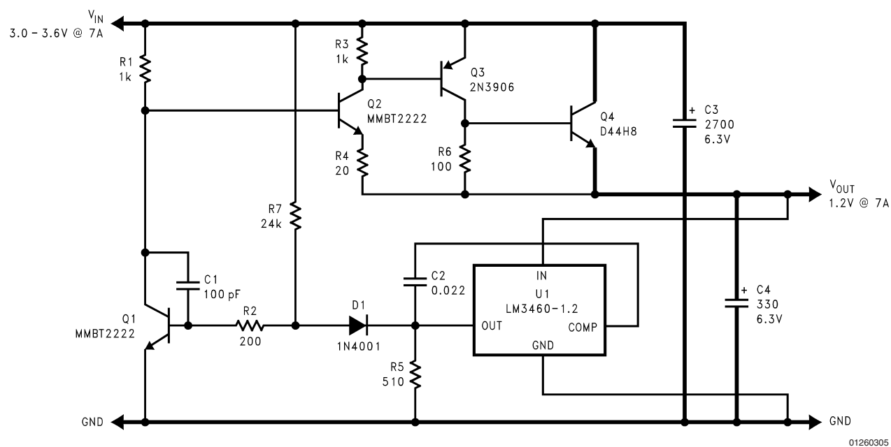
FIGURE 2. 1.2V Typical Application (See Application Information Section)
