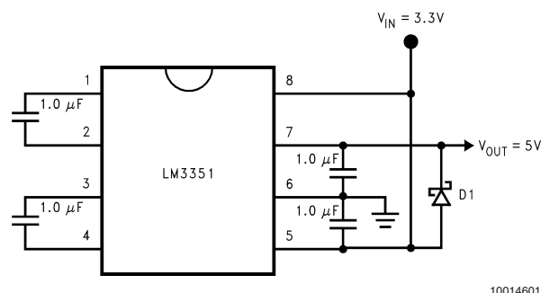
Step-Up Converter
