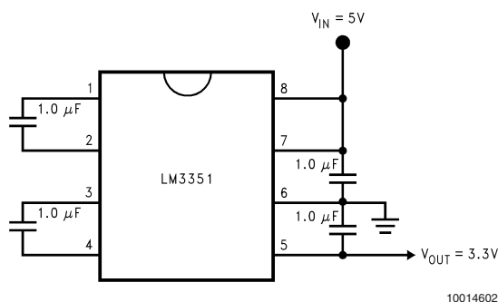
Step-Down Converter
