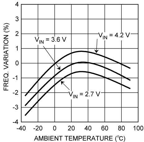
Switching Frequency Variation vs Temperature ( V_{OUT} = 1.5V , I_{OUT} = 200 mA )
