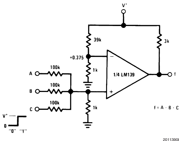
AND Gate
