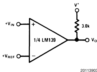
Basic Comparator
