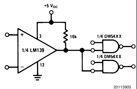
Driving TTL
