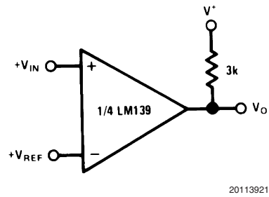
Basic Comparator
