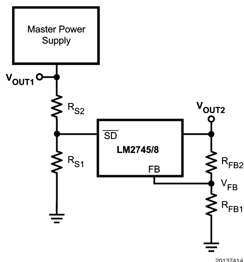
FIGURE 6. Sequencing Circuit
