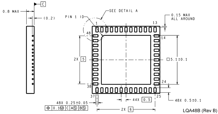
48-Lead LLP Package Order Number LM27262LQ NS Package Number LQA48B
