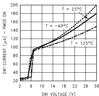
SWI Current vs. SWI Voltage (PMOS ON)
