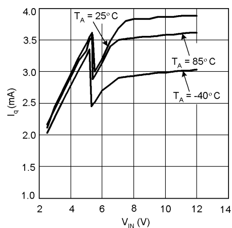
I_q vs V_{IN} (600 kHz, switching)
