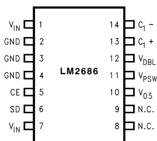
14-Pin TSSOP
