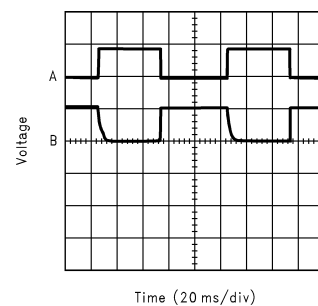
V_{O5} Response to SD (with 5mA Load)
