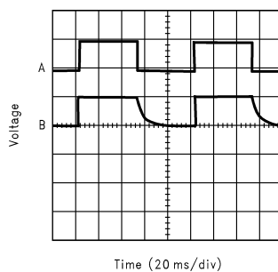
V_{PSW} Response to CE (with 5mA Load)
