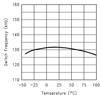
Switch Frequency vs. Temperature ( V_{IN} = 3.6\text{V} )
