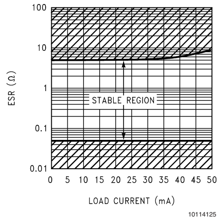
FIGURE 3. ESR Curve for C_{OUT} = 2.2\mu F
