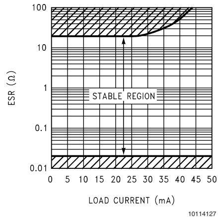
FIGURE 5. ESR Curve for C_{OUT} = 10\mu F
