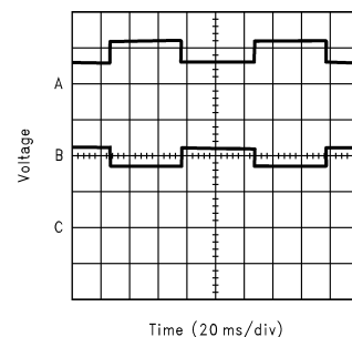
Line Transient Response (with 5mA Load)
