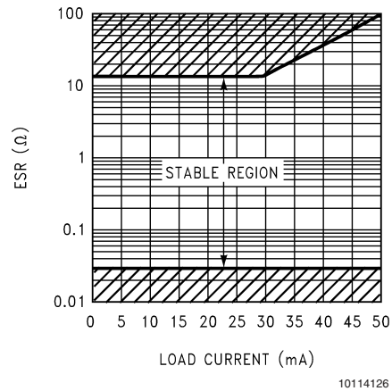
FIGURE 4. ESR Curve for C_{OUT} = 4.7\mu F
