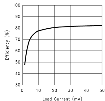
Efficiency vs Load Current ( V_{IN} = 3.0\text{V} )
