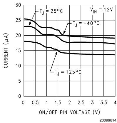
ON/OFF Pin Current (Sourcing)
