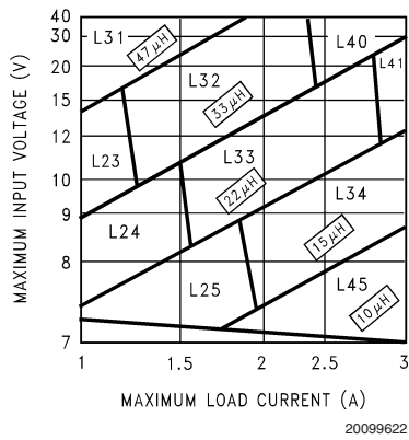
FIGURE 4. LM2676-5.0EP
