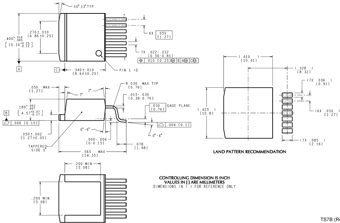
TO-263 Surface Mount Power Package NS Package Number TS7B
