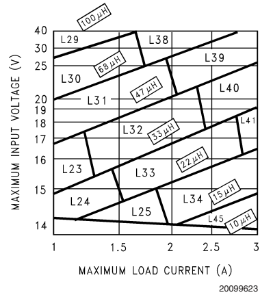
FIGURE 5. LM2676-12EP
