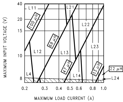
FIGURE 4. LM2675-3.3EP
