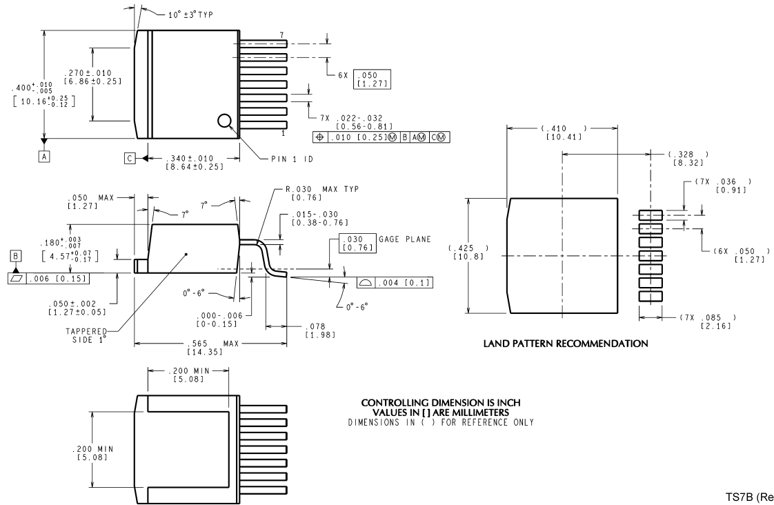
TO-263 Surface Mount Power Package NS Package Number TS7B
