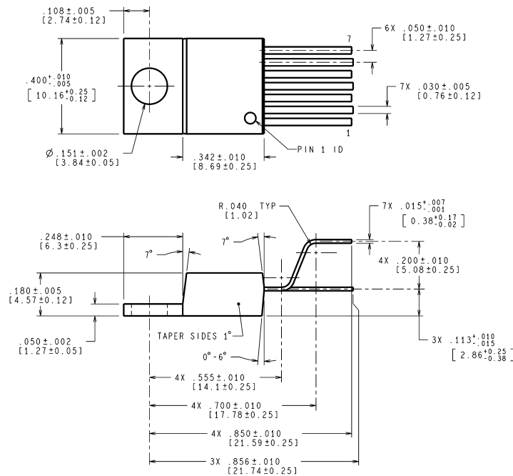
TO-263 Surface Mount Power Package NS Package Number TS7B
