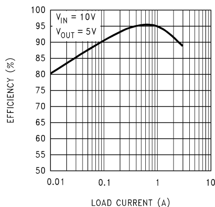
LM2650-ADJ Efficiency
