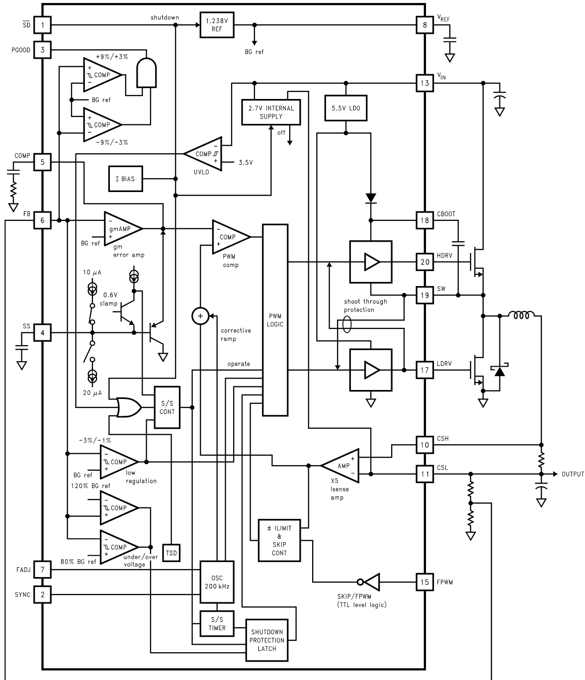
FIGURE 1. LM2631 Block Diagram
