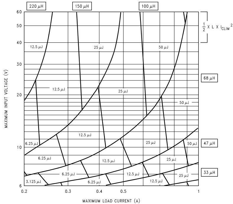
FIGURE 4. LM2590HV-3.3-AQ
