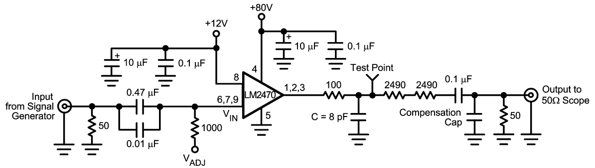
FIGURE 2. Test Circuit (One Channel)
