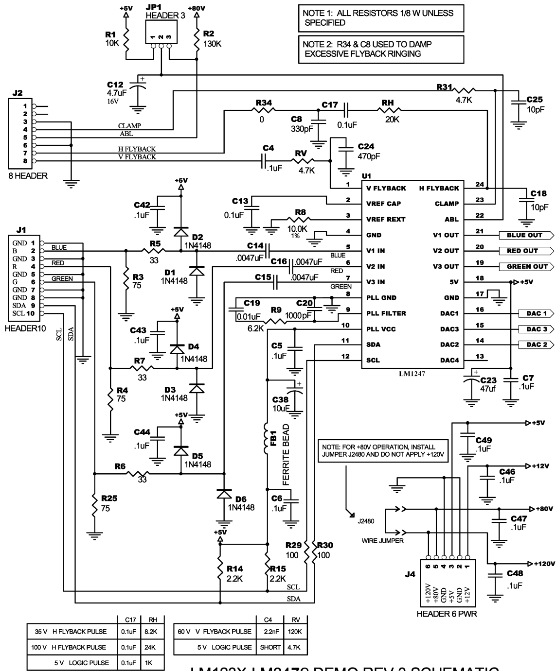
FIGURE 11. LM123X/LM124X - LM246X Demonstration Board Schematic
