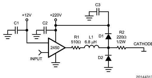
FIGURE 13. One Channel of the LM2450 with the Recommended Application Circuit
