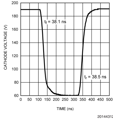
FIGURE 12. LM2450 Cathode Response
