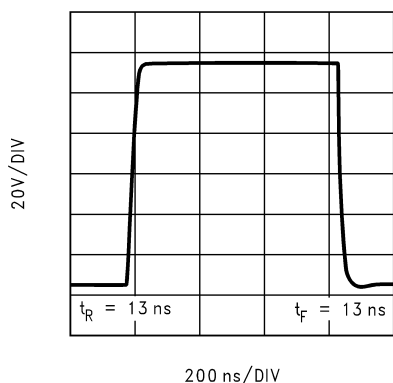
FIGURE 5. LM2426 Pulse Response
