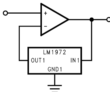
FIGURE 10. Digitally-Controlled Logarithmic Gain Amplifier Circuit
