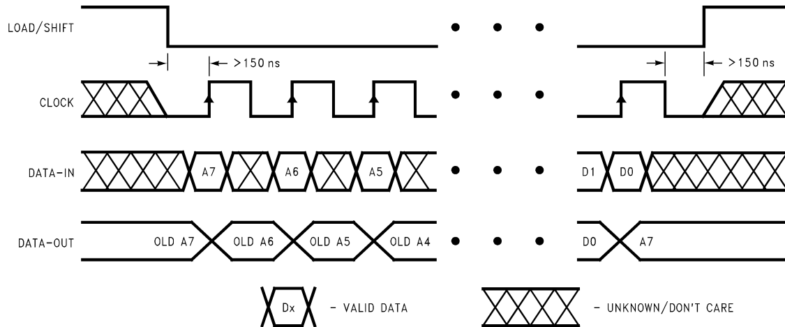
FIGURE 2. Timing Diagram
