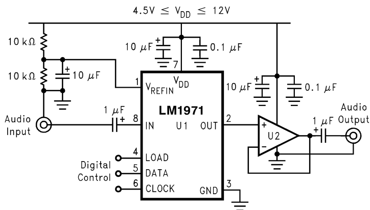
FIGURE 1. Typical Audio Attenuator Application Circuit
