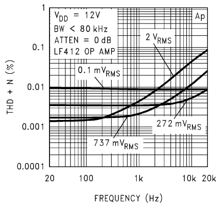
THD + N vs Freq and Amp
