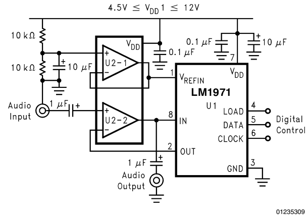
FIGURE 8. Logarithmic Gain Amplifier Circuit
