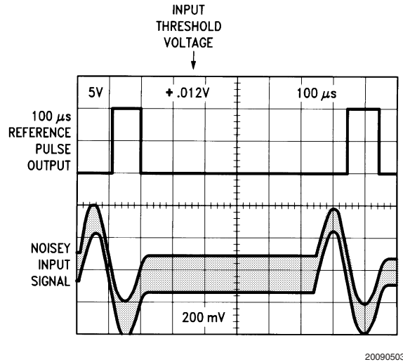
FIGURE 2. LM1815EP Oscillograms
