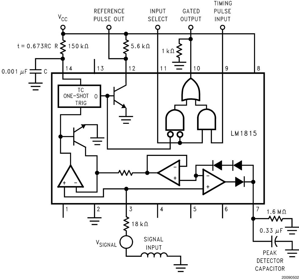
FIGURE 1. LM1815EP Adaptive Sense Amplifier
