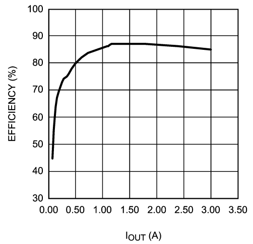
Efficiency vs I_{OUT} ( V_{IN} = 5V , V_{OUT} = 2.5V )
