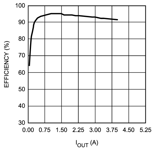
Efficiency vs I_{OUT} ( V_{IN} = 5V , V_{OUT} = 3.3V )
