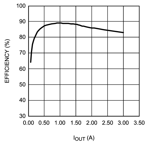
Efficiency vs I_{OUT} ( V_{IN} = 3.3V , V_{OUT} = 0.8V )
