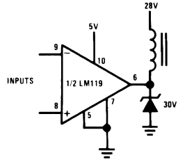
Relay Driver
