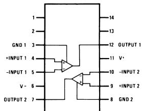
Top View See NS Package Number J14A
