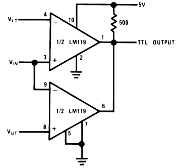
Window Detector
