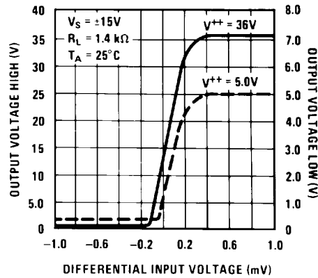
Transfer Function
