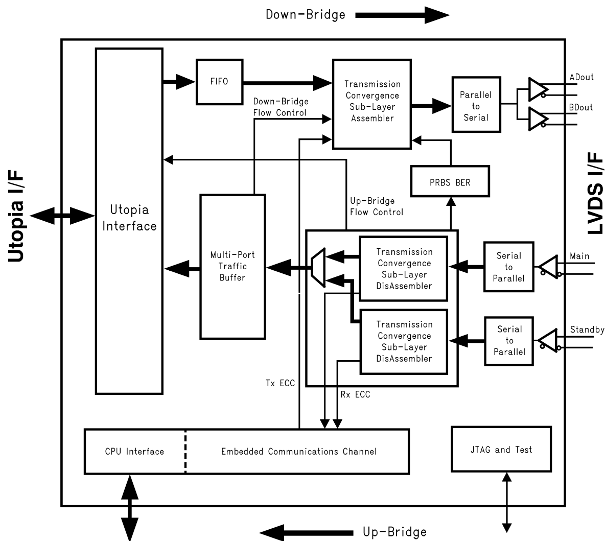
FIGURE 1. DS92UT16 Block Diagram
