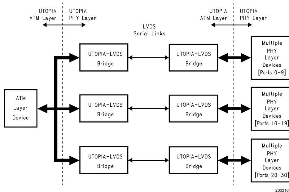
FIGURE 5. Multi-Bridge System Example
