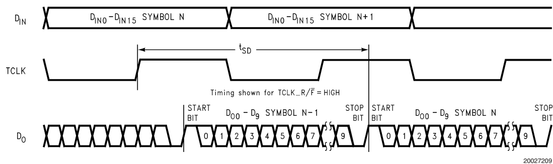
FIGURE 7. Serializer Delay
