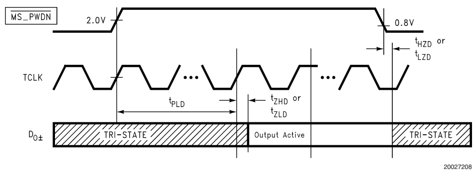
FIGURE 6. Serializer PLL lock Time and \overline{\text{MS\_PWDN}} TRI-STATE Delays
