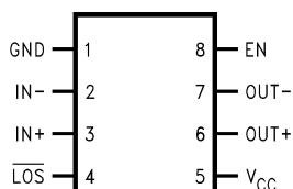
SOIC - Top View
