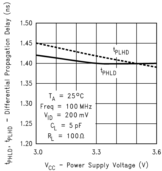
Differential Propagation Delay vs Power Supply Voltage
