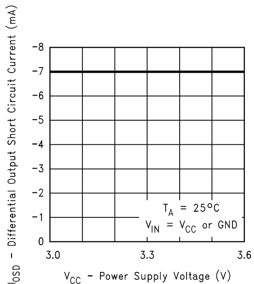
Differential Output Short Circuit Current vs Power Supply Voltage
