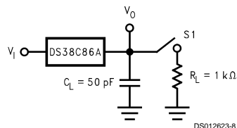
FIGURE 5. Receiver: Propagation Delay Set-Up
