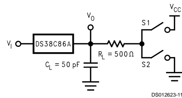
FIGURE 8. Receiver: Enable/Disable Set-Up
