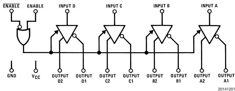
Dual-In-Line Package
