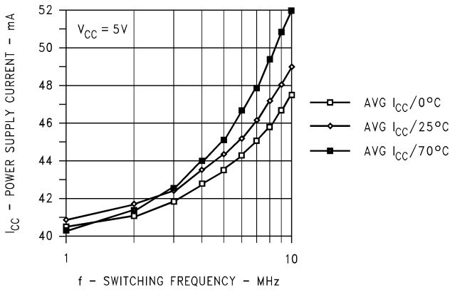
DS26LS31MQMLCN Unloaded I_C vs Frequency vs T_A
