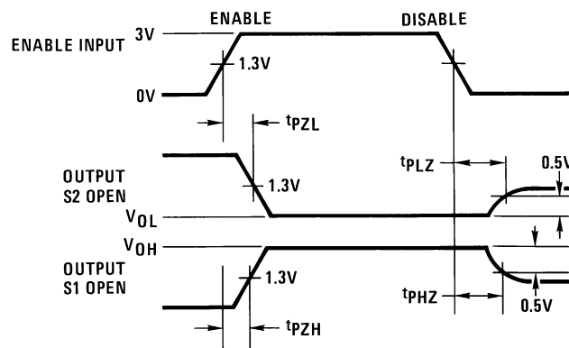
FIGURE 2. Propagation Delays
