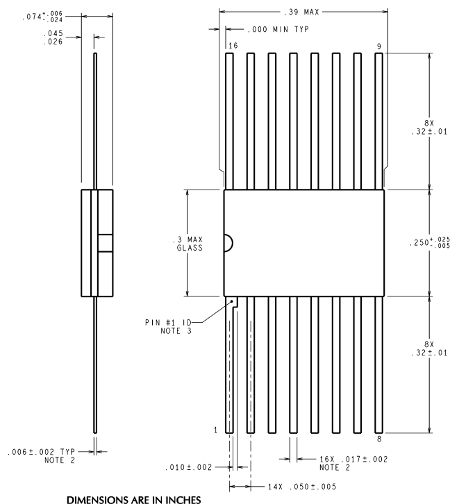
16 Lead Ceramic Flatpak (F) NS Package Number W16A
