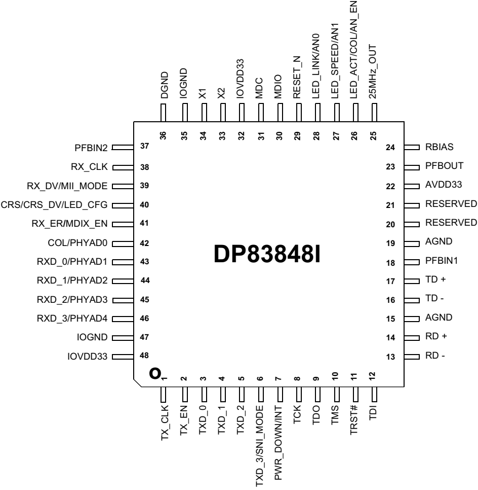
Top View NS Package Number VBH48A
