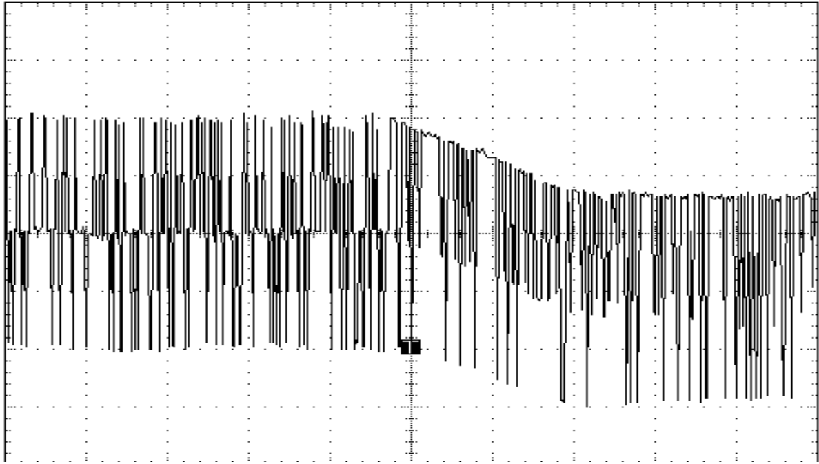
Figure 9. 100BASE-TX BLW Event
