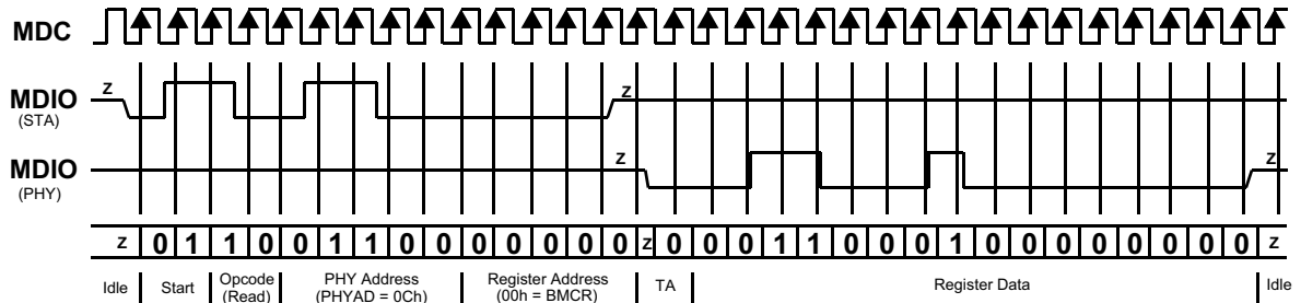
Figure 4. Typical MDC/MDIO Read Operation
