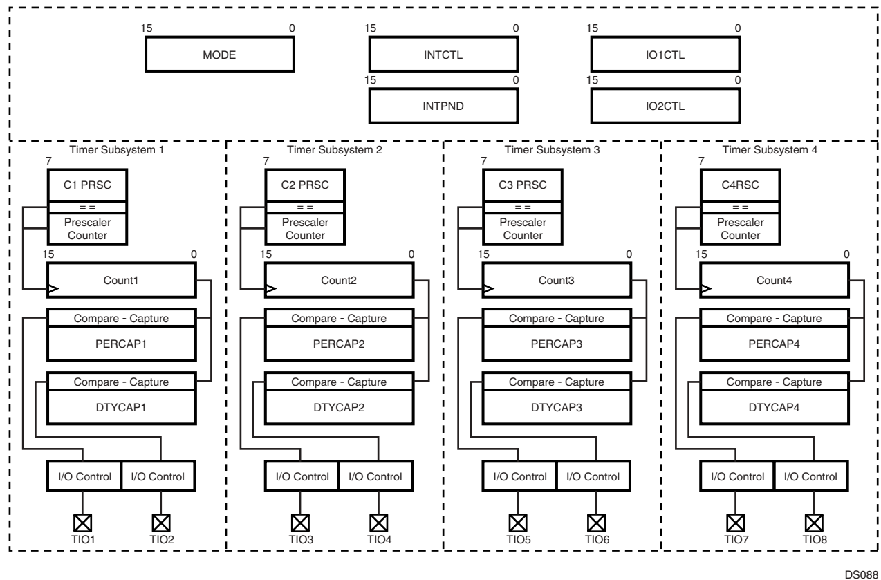
Figure 53. Versatile Timer Unit Block Diagram
