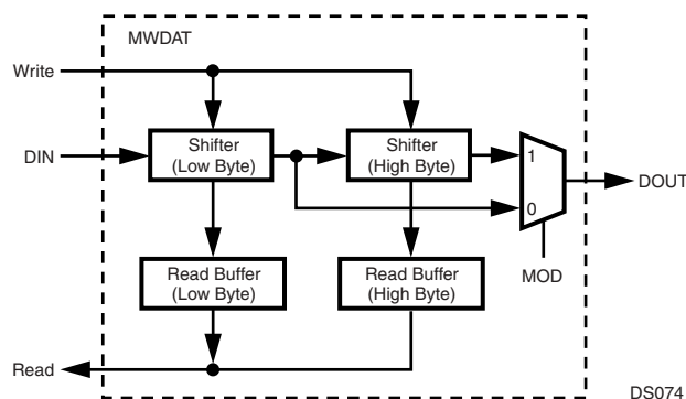
Figure 41. MWDAT Register
