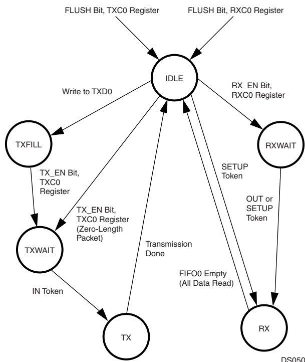
Figure 13. Endpoint 0 Operation
