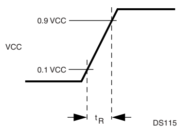
Figure 62. Power-On Reset
