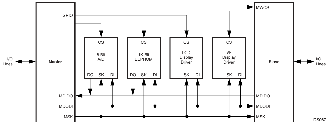
Figure 34. Microwire Interface
