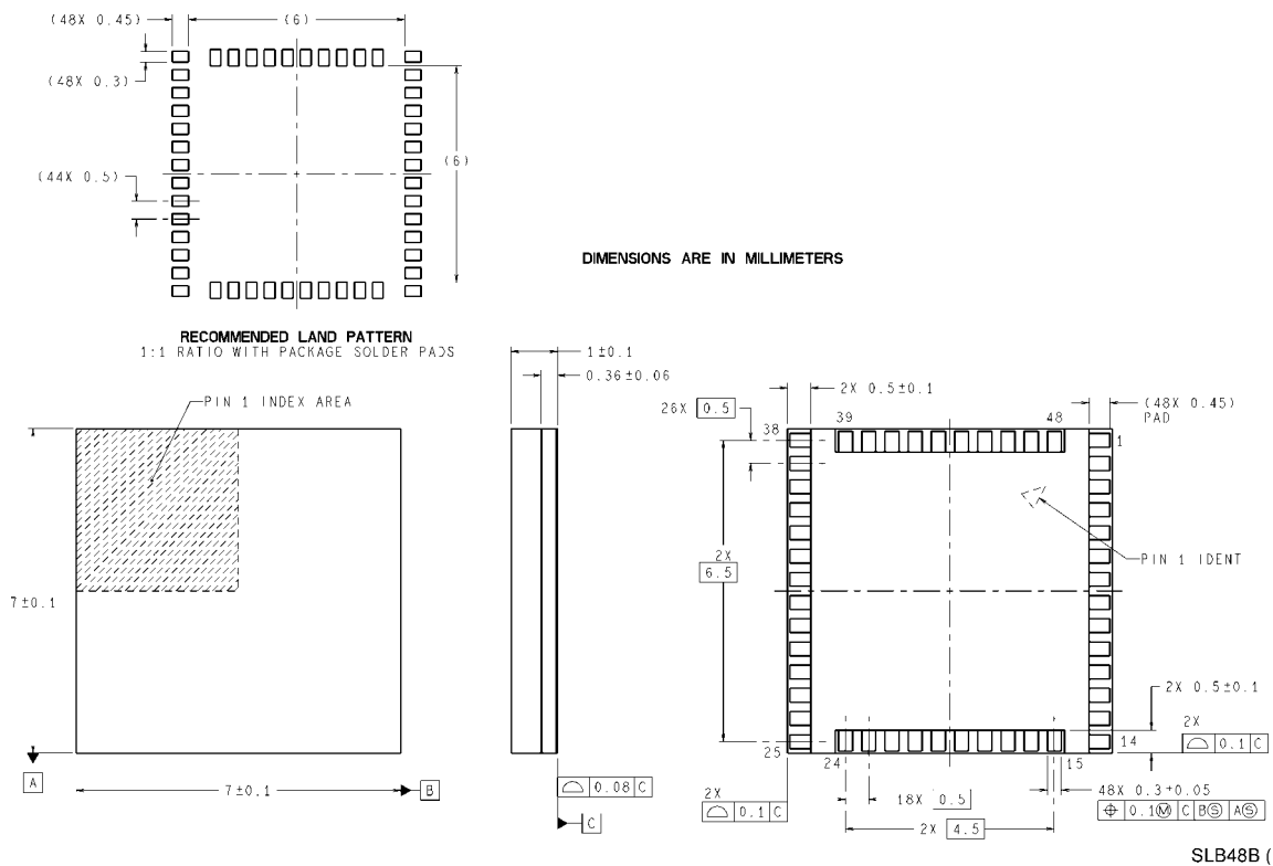
Figure 87. 48-Pin CSP Package
