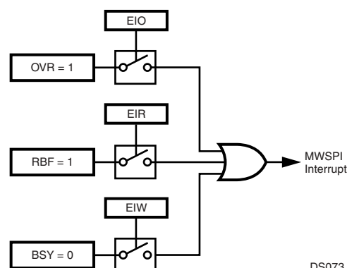
Figure 40. MWSPi Interrupts
