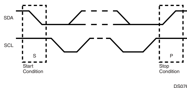
Figure 43. Start and Stop Conditions
