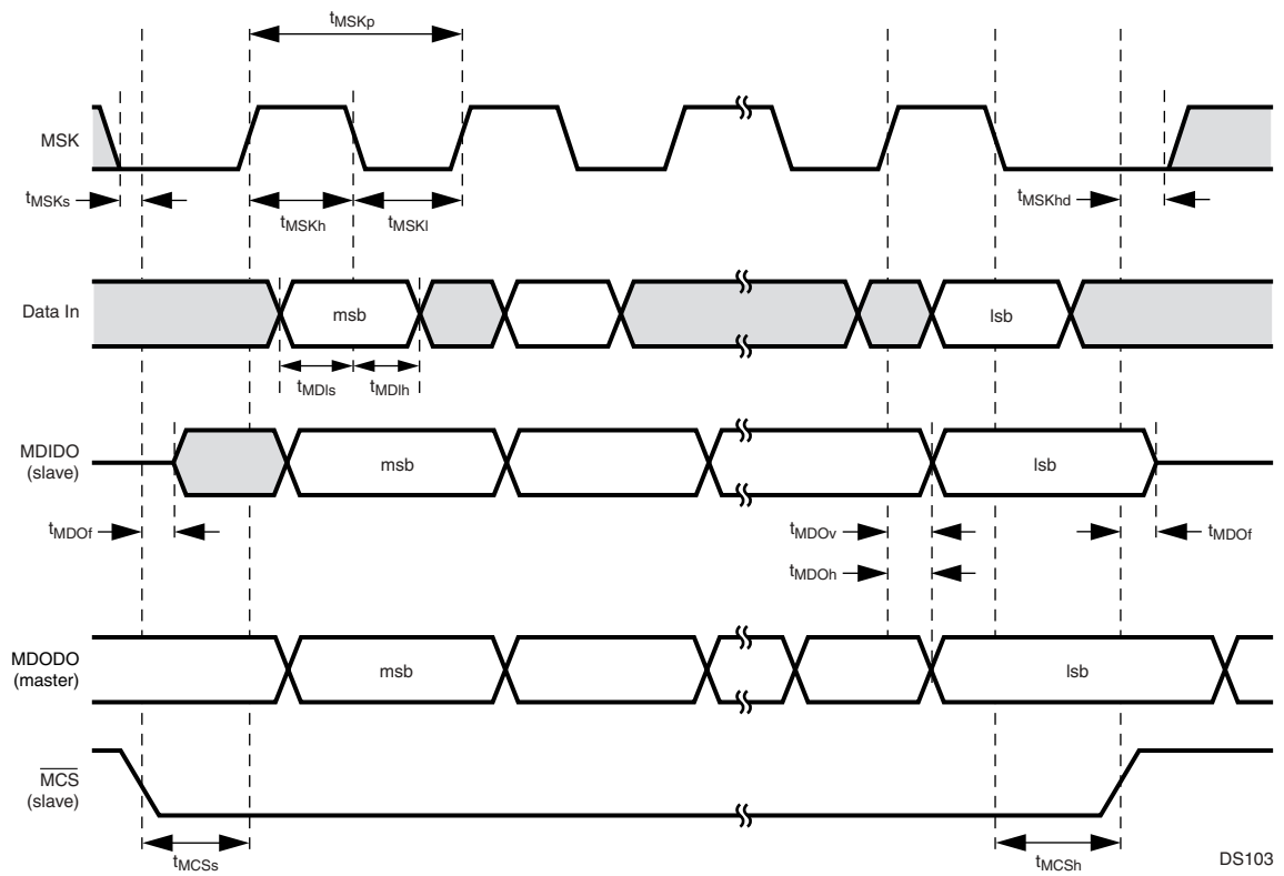
Figure 70. Microwire Transaction Timing, Alternate Mode, SCIDL = 0
