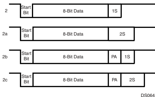
Figure 65. 8-Bit Data Frame Options
