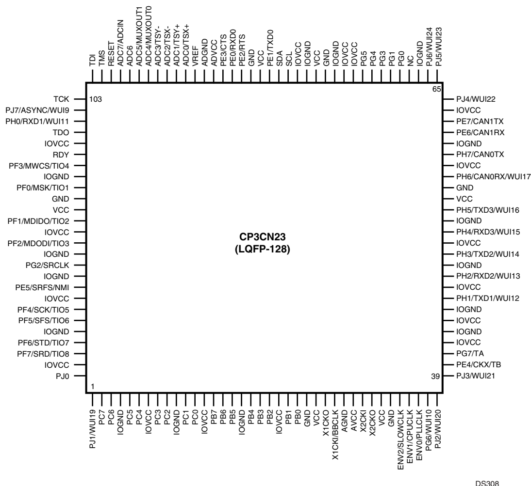
Figure 121. CP3CN23 in the LQFP-128 Package (Top View)
