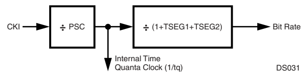
Figure 32. CAN Prescaler
