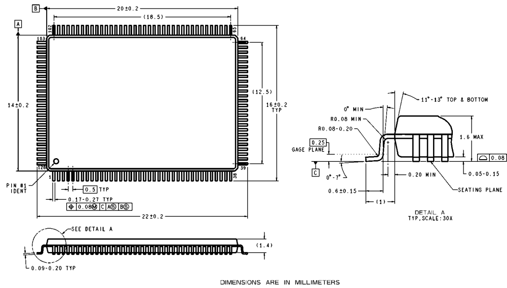
Figure 123. LQFP-128 Package
