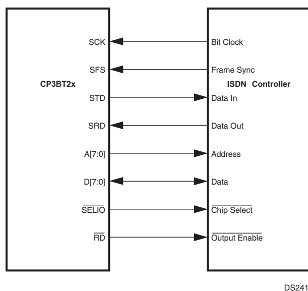
Figure 59. CP3CN23/ISDN Controller Connections
