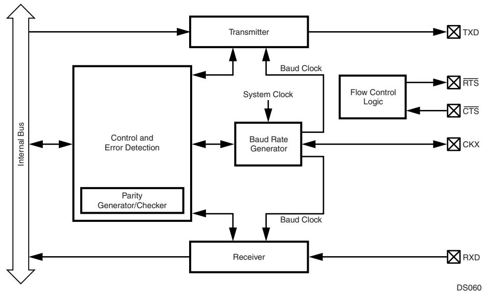
Figure 61. UART Block Diagram
