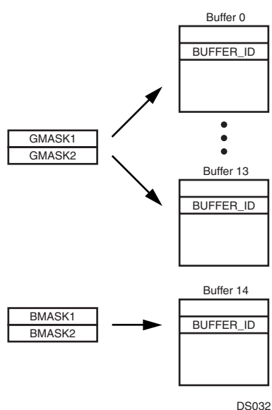
Figure 33. Acceptance Filtering
