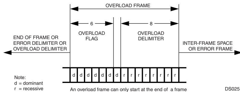
Figure 26. Overload Frame
