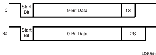
Figure 66. 9-bit Data Frame Options
