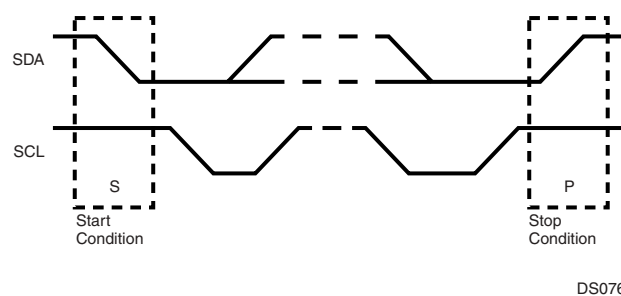
Figure 77. Start and Stop Conditions
