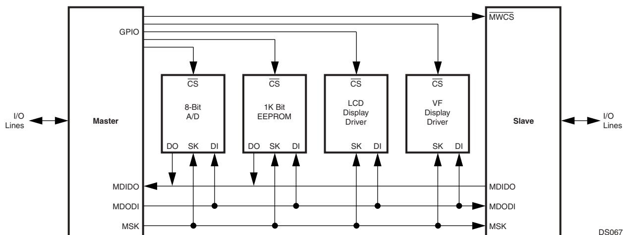
Figure 68. Microwire Interface
