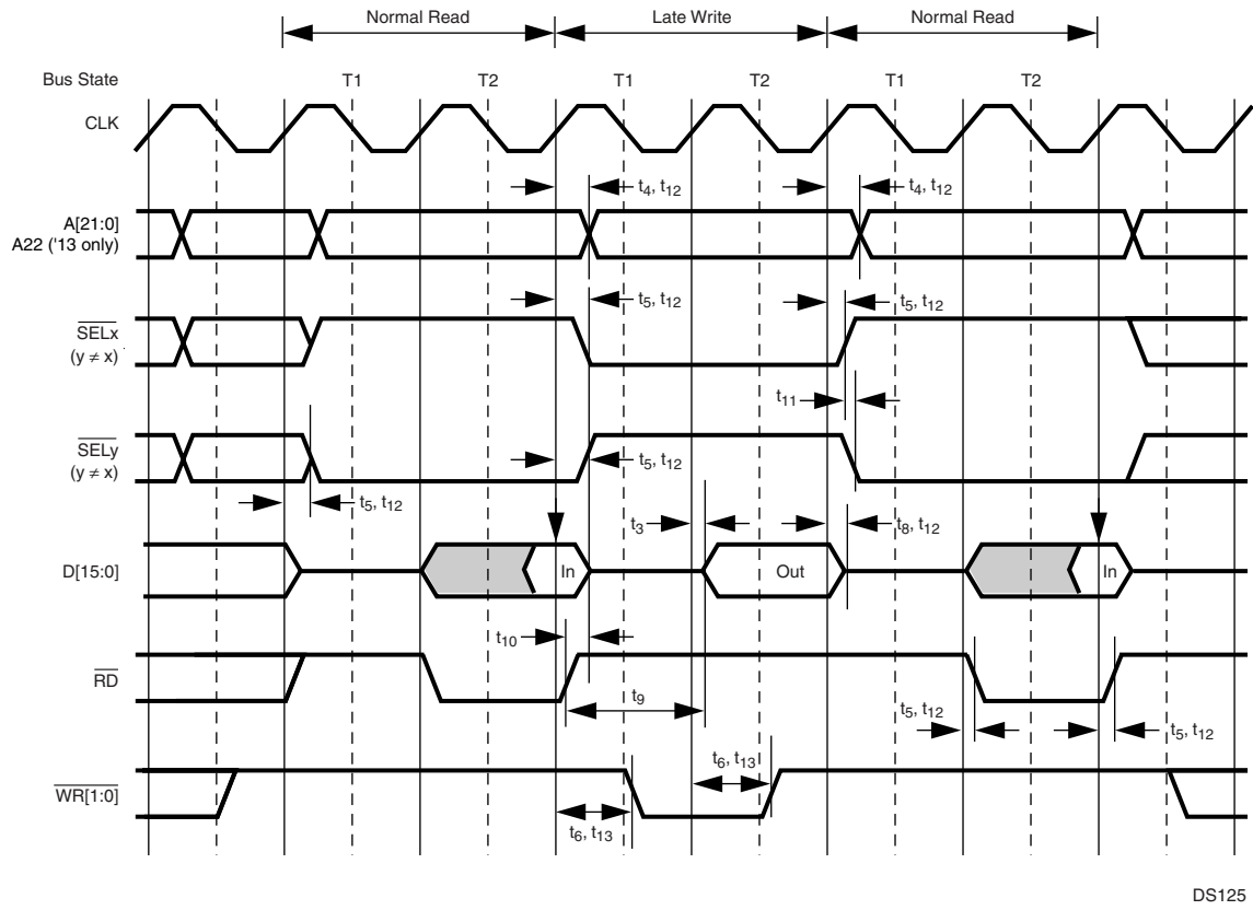
Figure 117. Late Write Between Normal Read Cycles (No Wait States)
