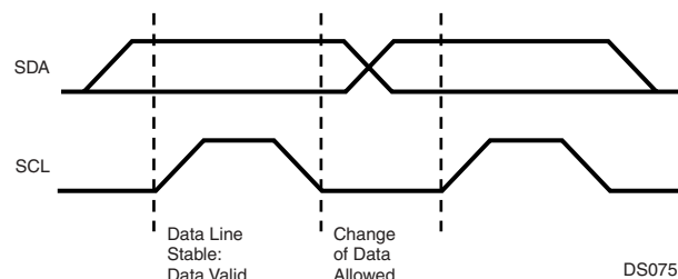
Figure 76. Bit Transfer
