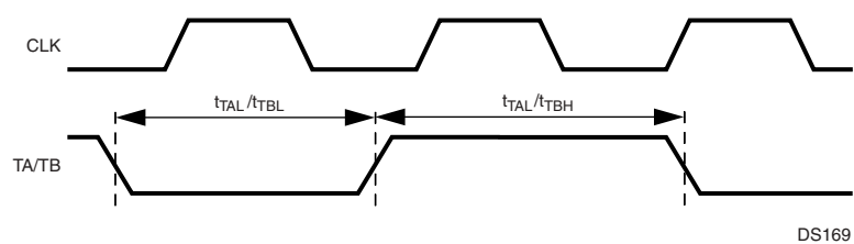
Figure 114. Multi-Function Timer Input Timing
