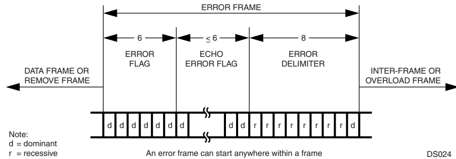
Figure 25. Error Frame
