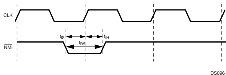
Figure 96. \overline{\text{NMI}} Signal Timing
