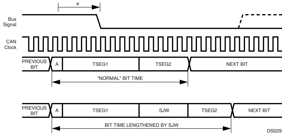
Figure 30. Resynchronization ( e > SJW )
