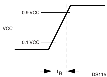
Figure 98. Power-On Reset
