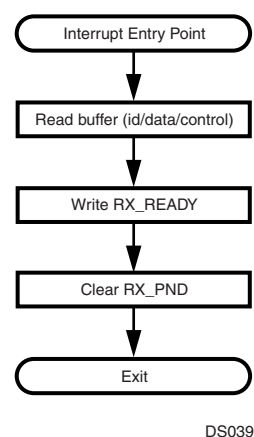
Figure 40. Buffer Read Routine (BUFFLOCK Enabled)
