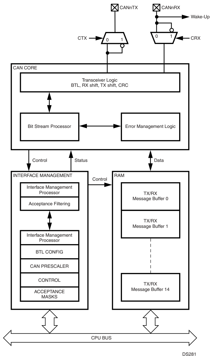
Figure 19. CAN Block Diagram
