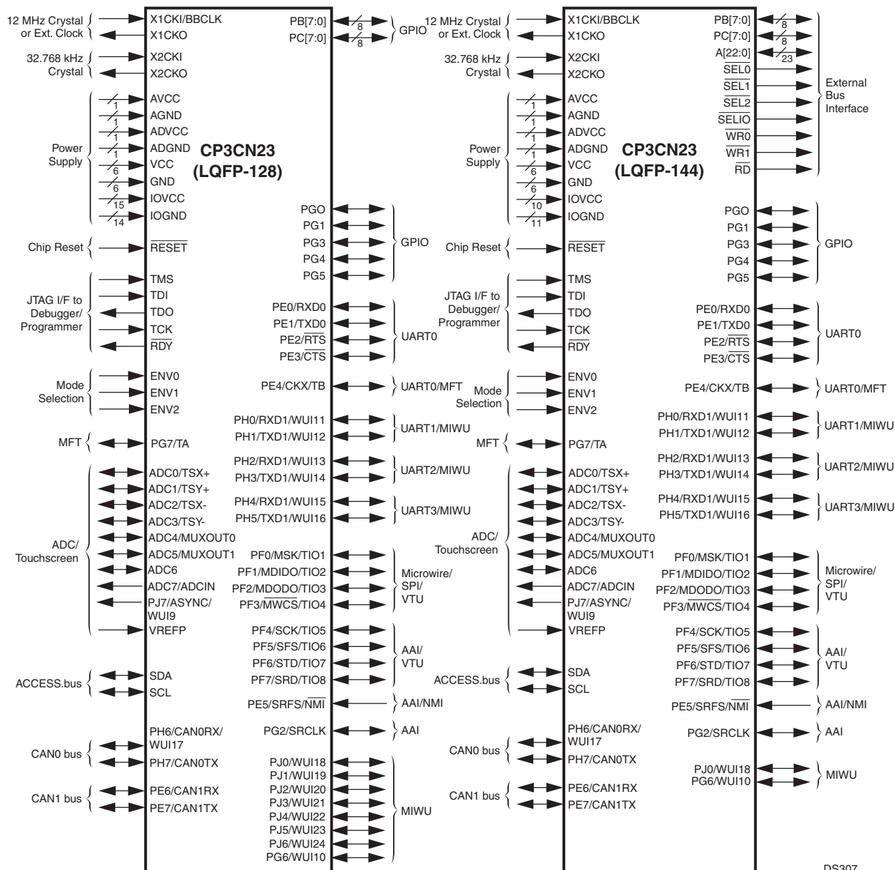
Figure 1. CP3CN23 Device Signals
