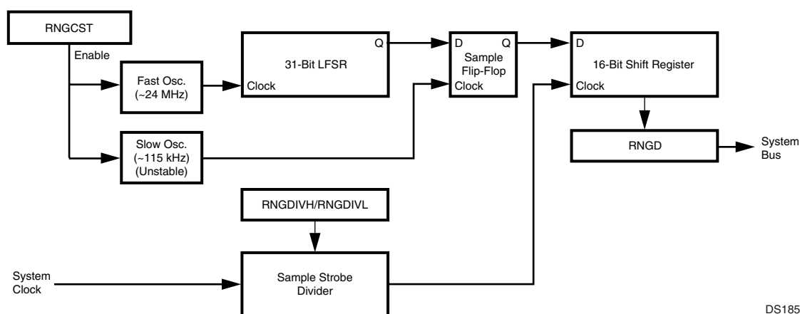
Figure 18. RNG Module Block Diagram
