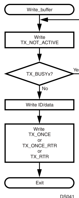
Figure 42. Buffer Write Routine
