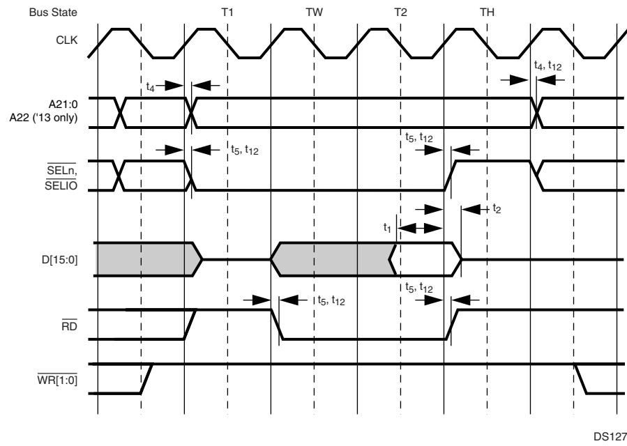
Figure 119. Normal Read Cycle (Wait Cycle Followed by Hold Cycle)
