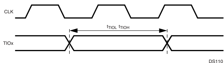
Figure 115. Versatile Timing Unit Input Timing
