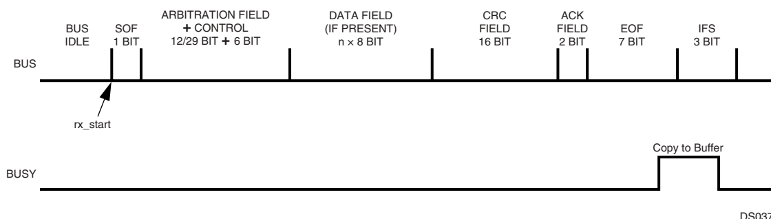
Figure 38. Receive Timing
