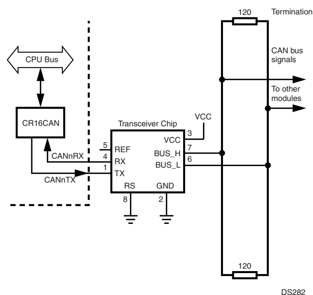
Figure 49. External Transceiver
