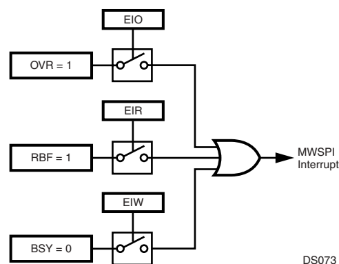
Figure 74. MWSPi Interrupts
