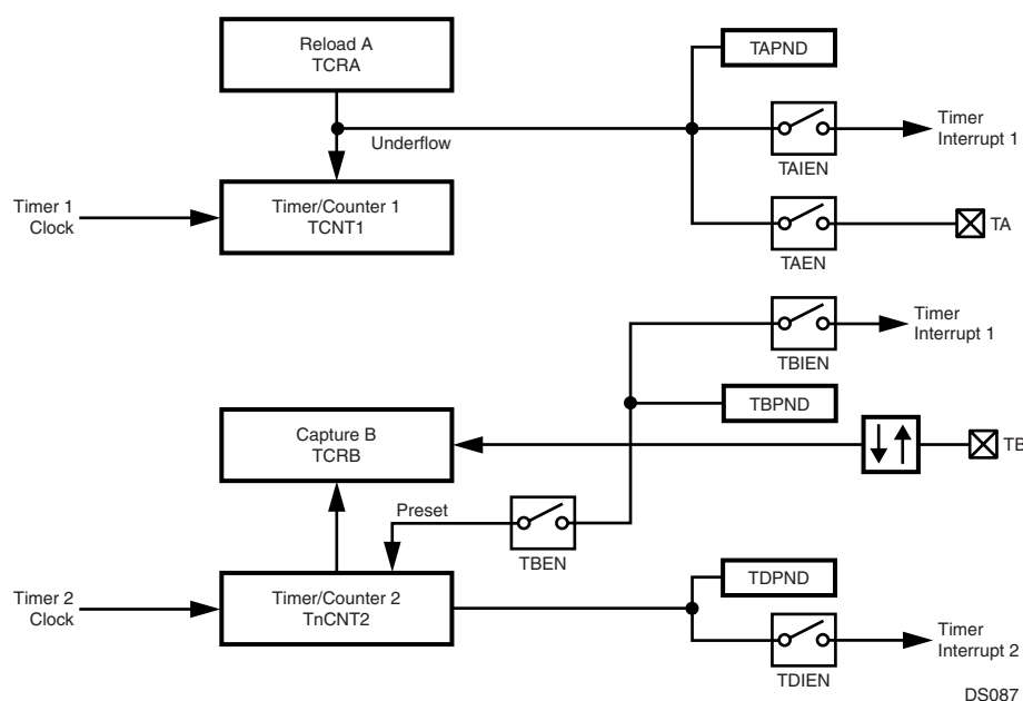
Figure 88. Input Capture Plus Timer Mode
