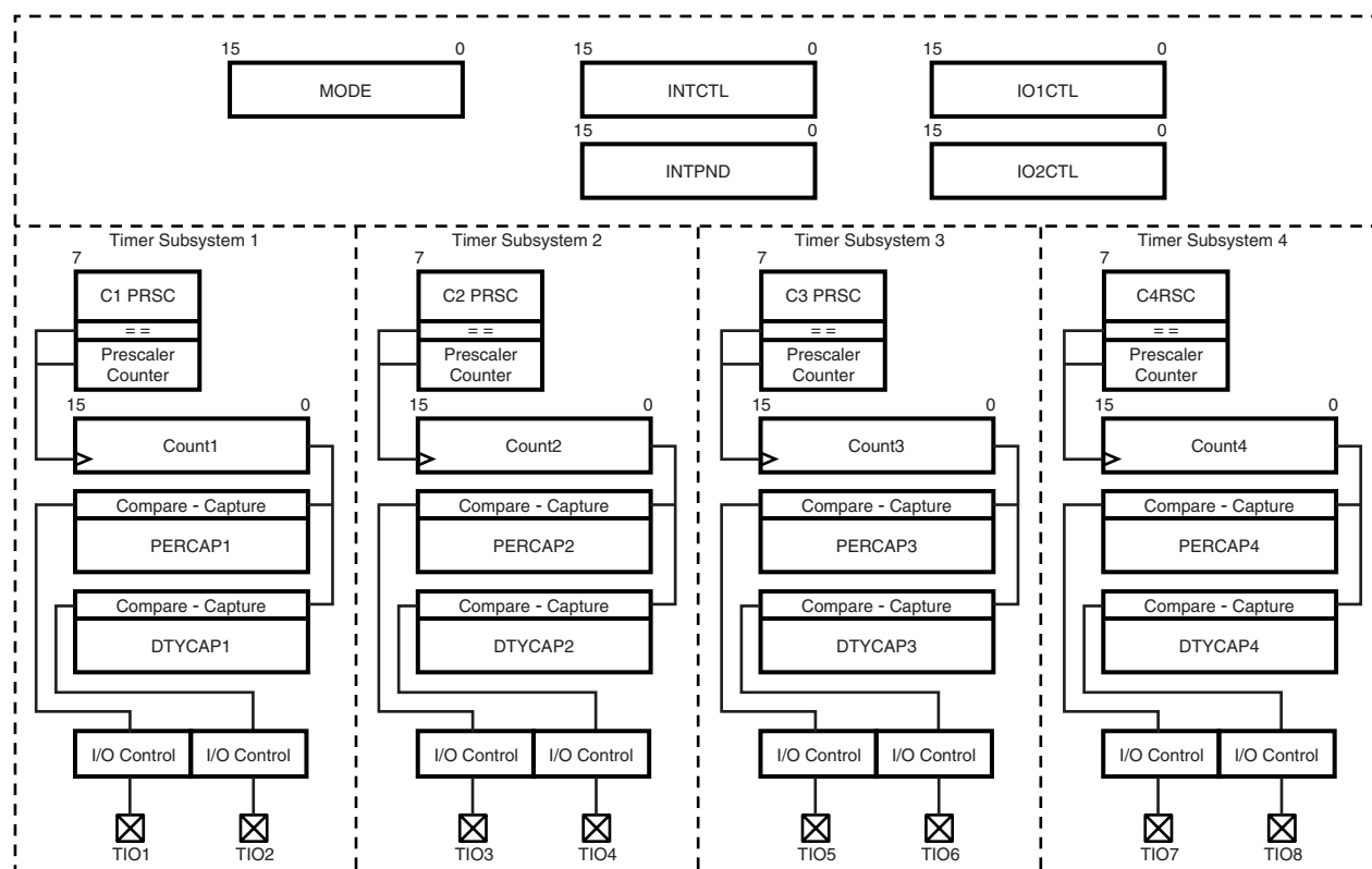
Figure 89. Versatile Timer Unit Block Diagram
