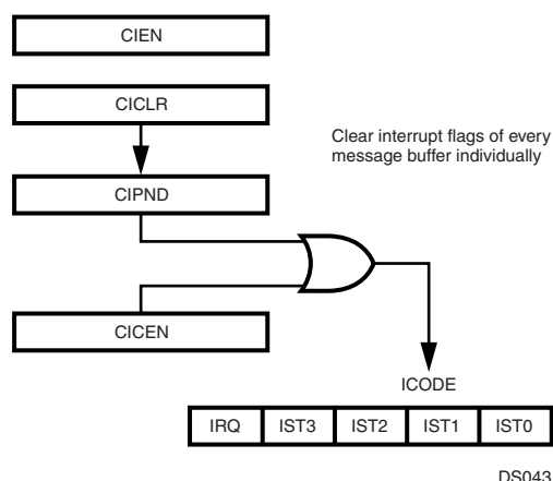
Figure 44. Interrupt Management
