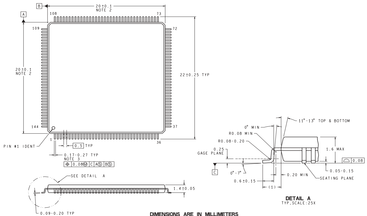
Figure 124. LQFP-144 Package
