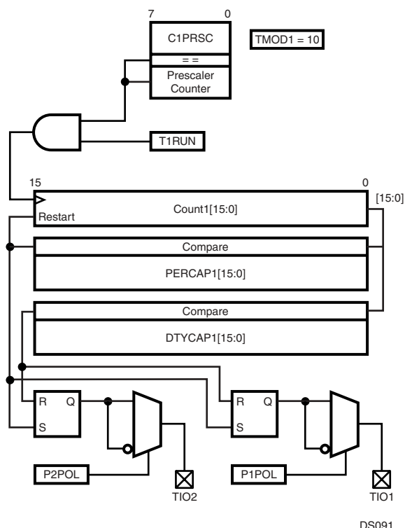
Figure 92. VTU 16-bit PWM Mode
