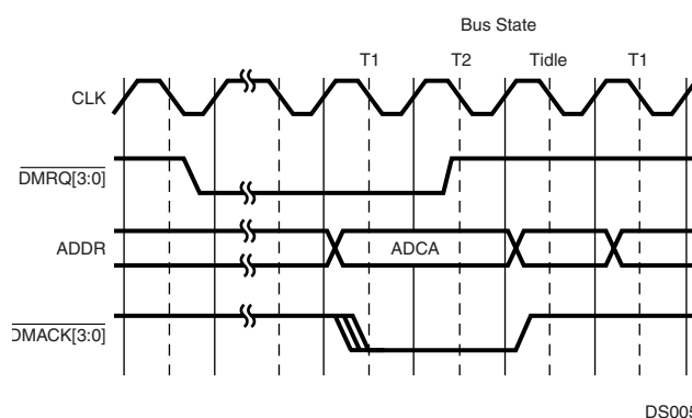
Figure 3. Direct DMA Cycle Followed by a CPU Cycle
