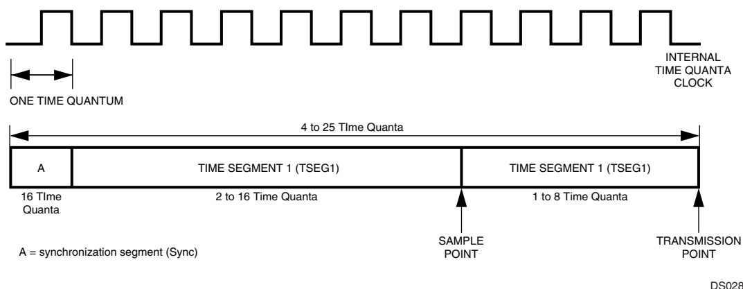
Figure 29. Bit Timing
