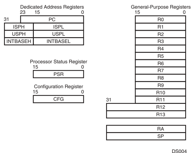
Figure 2. CPU Registers
