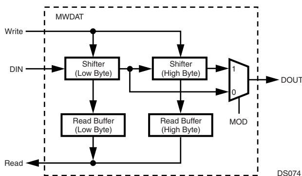
Figure 81. MWDAT Register
