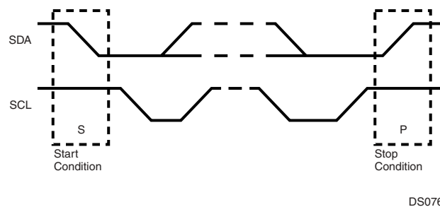
Figure 83. Start and Stop Conditions
