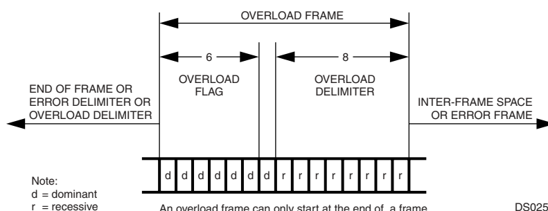
Figure 32. Overload Frame
