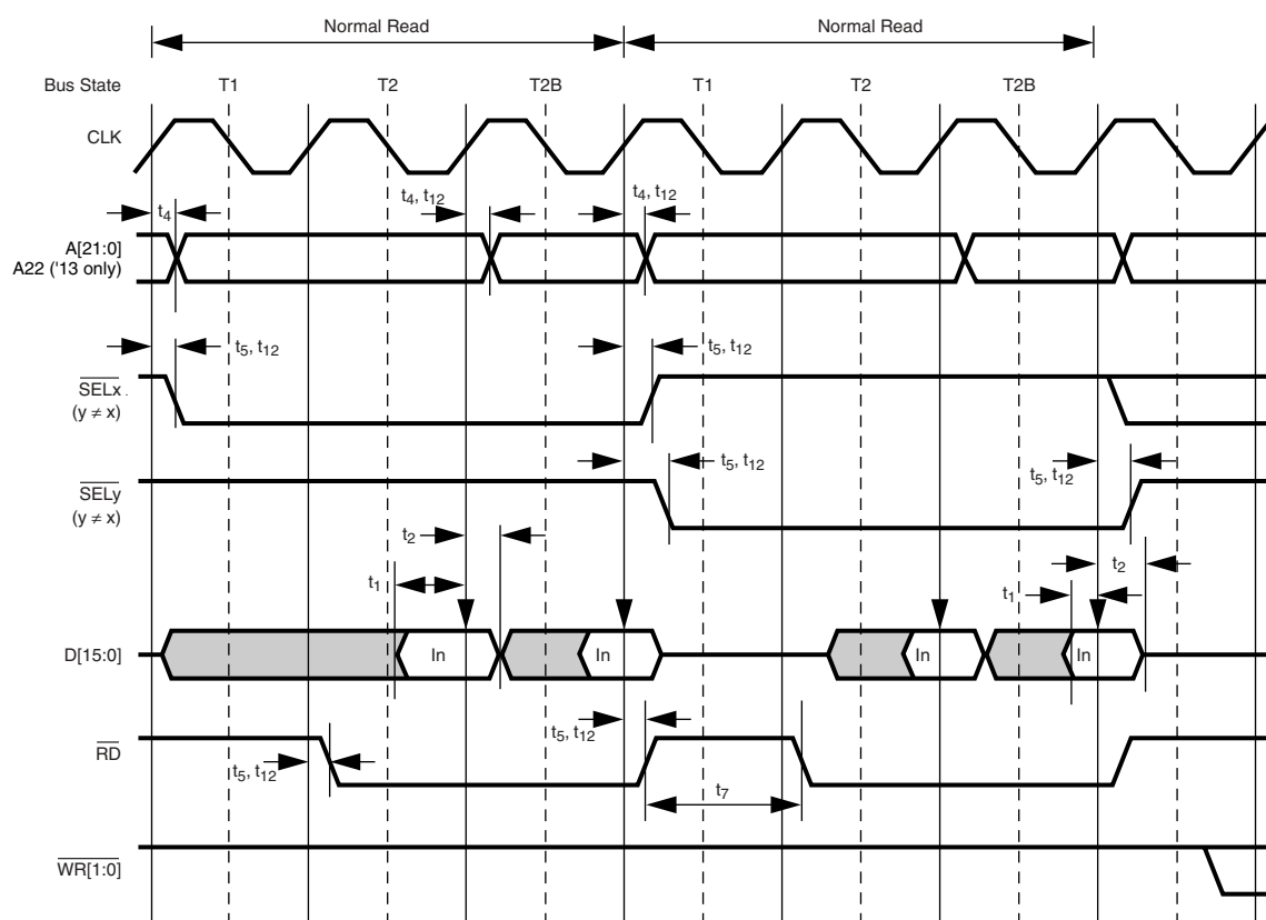
Figure 124. Consecutive Normal Read Cycles (Burst, No Wait States)
