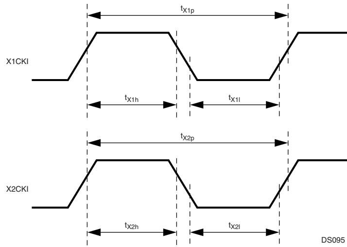
Figure 101. Clock Timing
