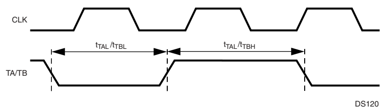
Figure 120. Multi-Function Timer Input Timing
