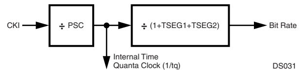
Figure 38. CAN Prescaler
