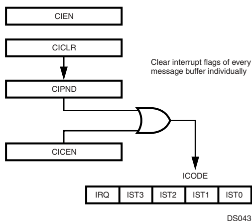
Figure 50. Interrupt Management
