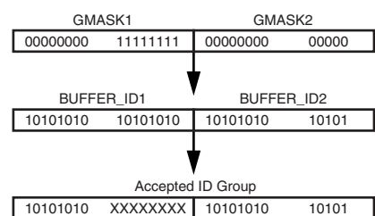
Figure 41. Acceptance of a Group of Identifiers
