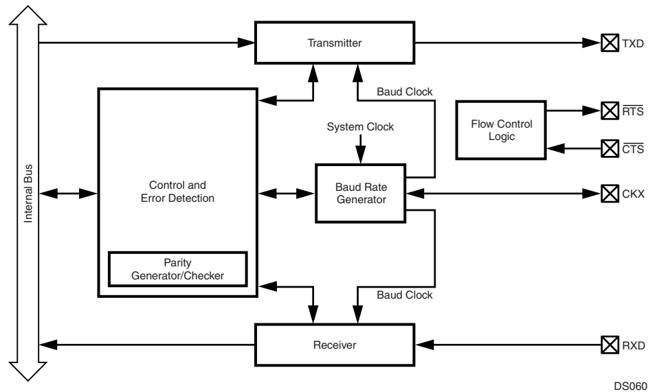
Figure 67. UART Block Diagram
