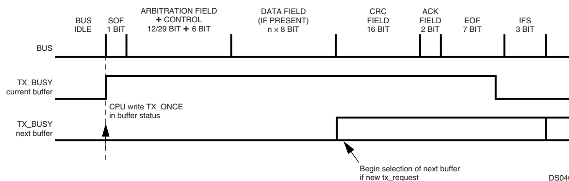
Figure 47. Data Transmission
