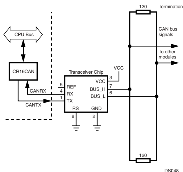
Figure 55. External Transceiver
