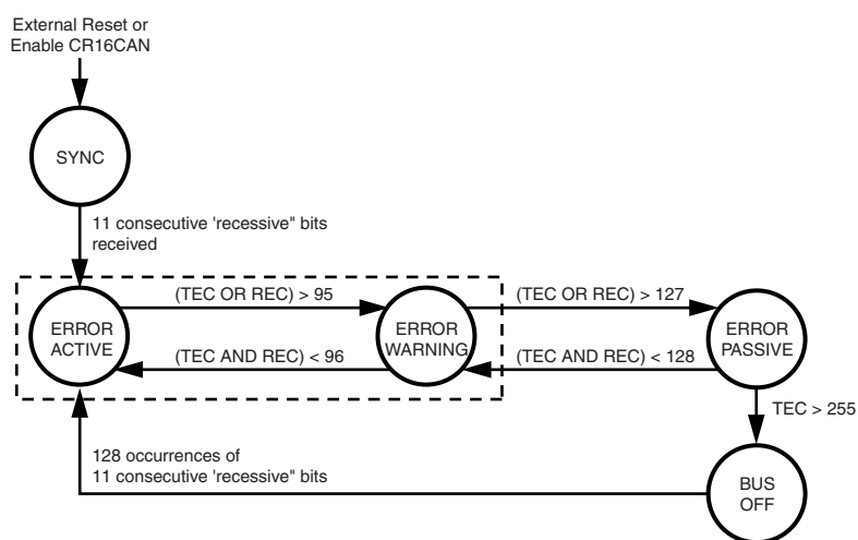
Figure 34. Bus States
