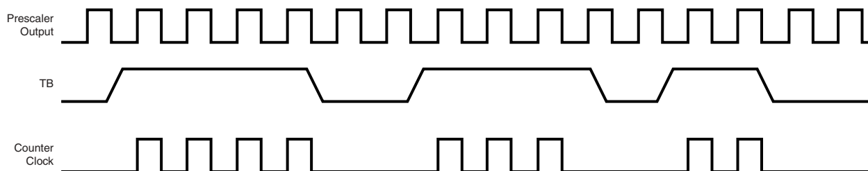
Figure 90. Pulse-Accumulate Mode
