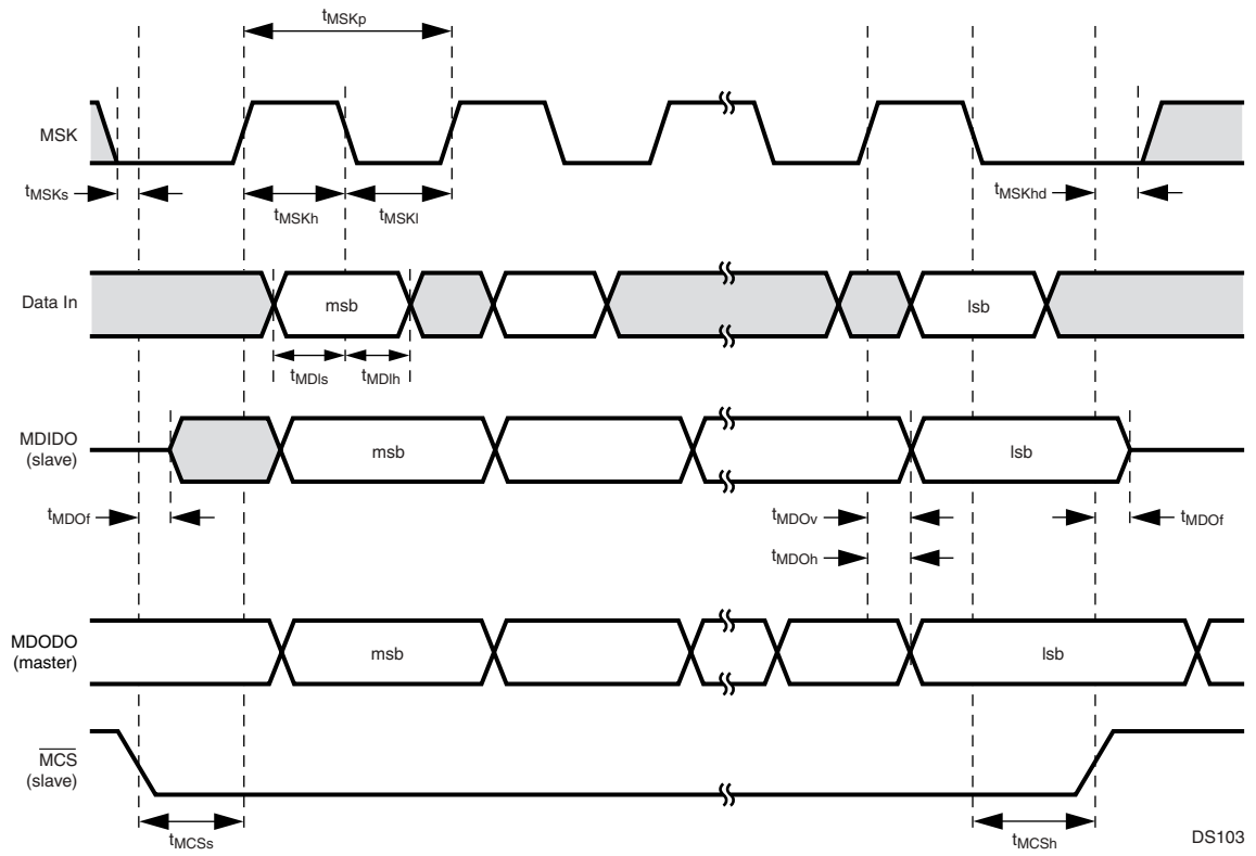
Figure 113. Microwire Transaction Timing, Alternate Mode, SCIDL = 0
