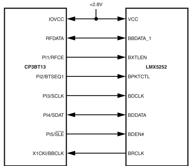
Figure 13. LMX5252 Interface
