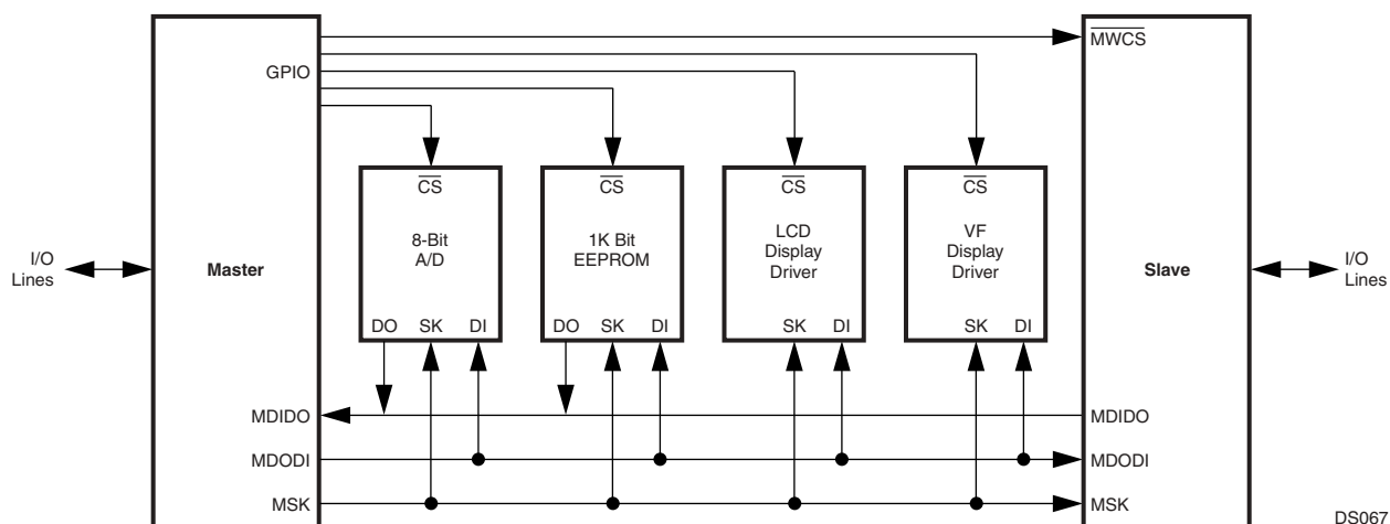
Figure 74. Microwire Interface
