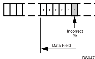
Figure 54. EBID Example
