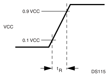
Figure 104. Power-On Reset
