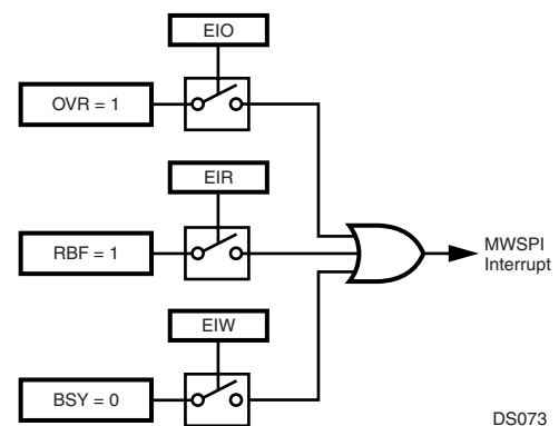
Figure 53. MWSPI Interrupts
