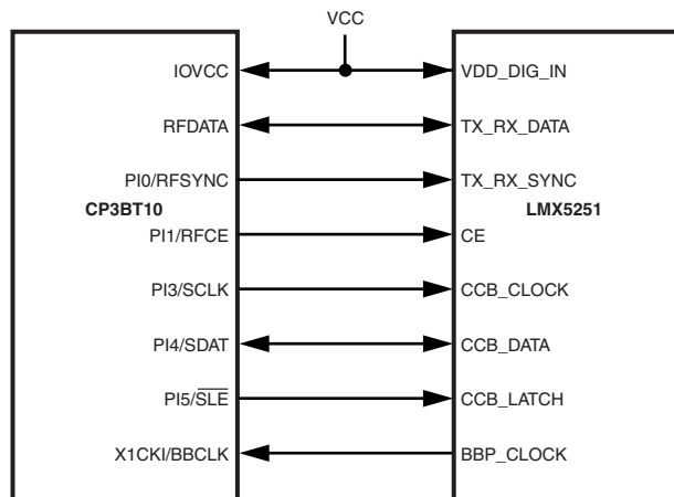
Figure 12. LMX5251 Interface
