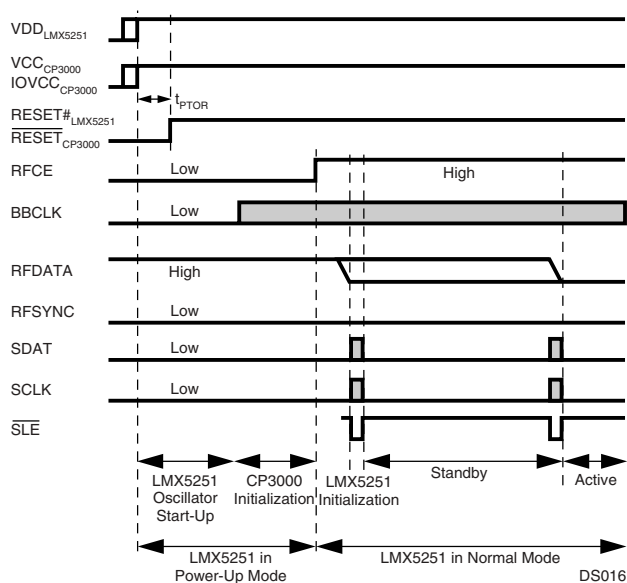
Figure 21. LMX5251 Power-Up Sequence
