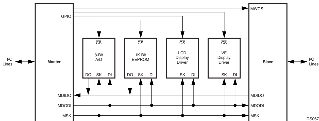
Figure 47. Microwire Interface
