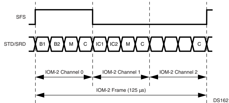
Figure 38. IOM-2 Frame Structure
