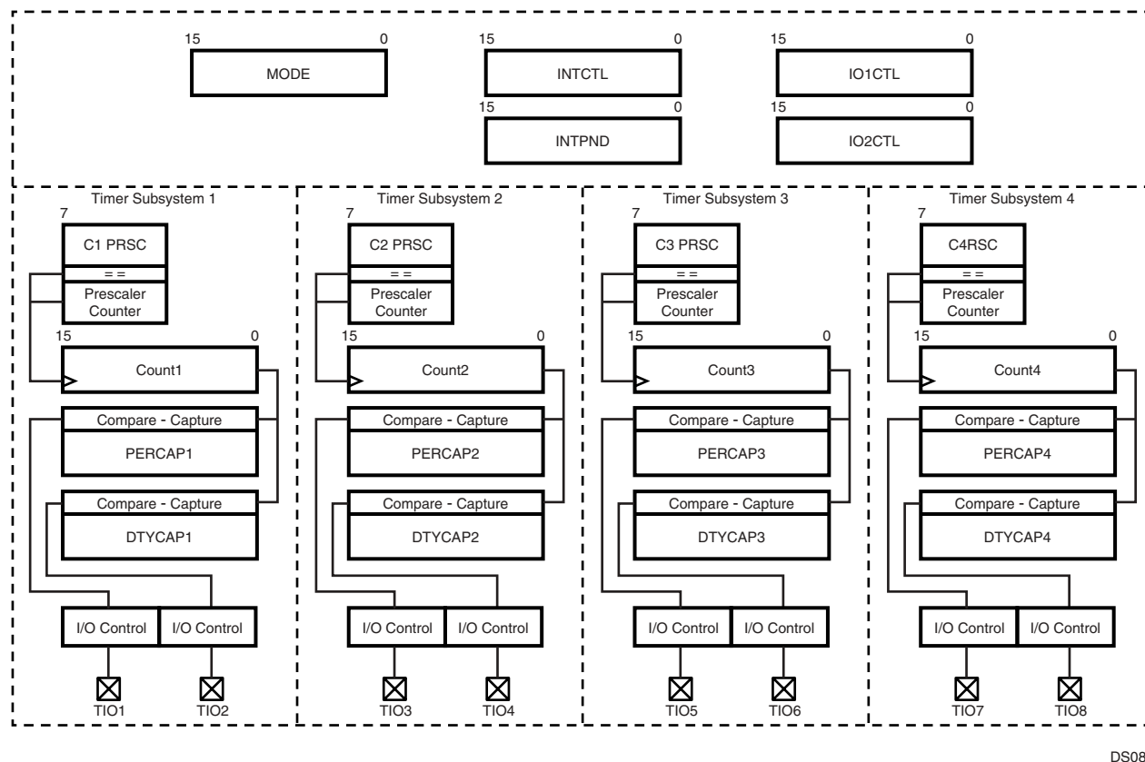
Figure 66. Versatile Timer Unit Block Diagram
