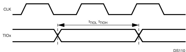
Figure 91. Versatile Timing Unit Input Timing
