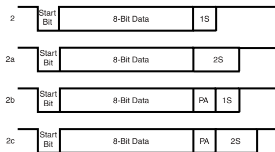
Figure 44. 8-Bit Data Frame Options
