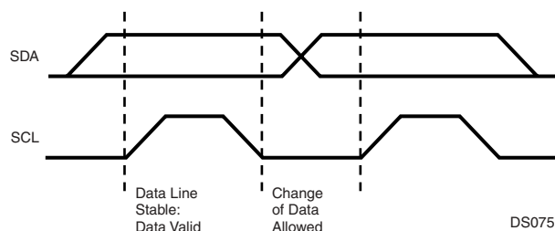
Figure 55. Bit Transfer
