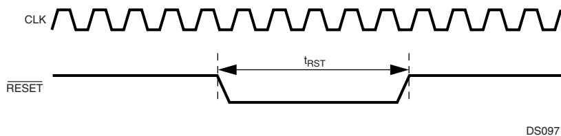
Figure 74. Non-Power-On Reset
