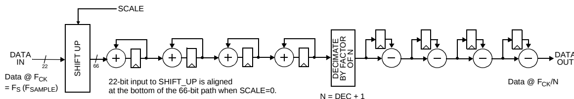
Figure 20. Four-stage decimate by N CIC filter
