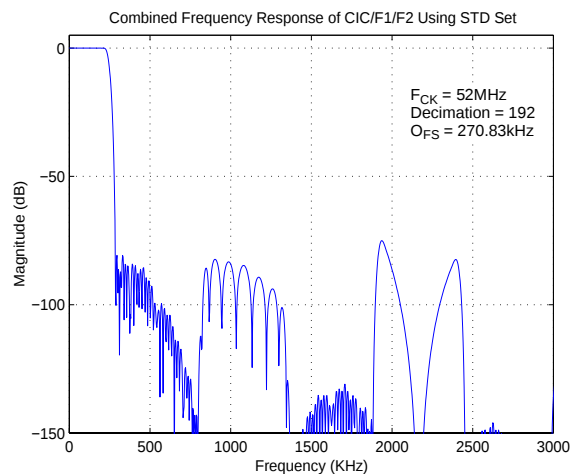
Figure 25. CIC, F1, & F2 STD frequency response
