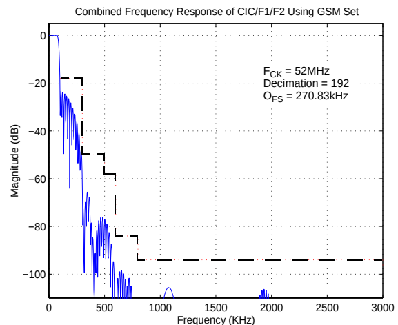
Figure 27. CIC, F1, & F2 GSM frequency response
