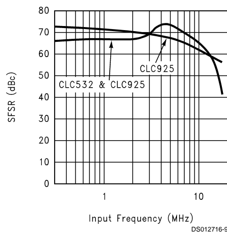
SFRD vs. Input Frequency
