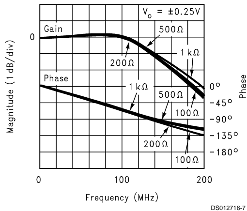
Small Signal Gain/Phase vs. Load with Recommended C_{COMP}
