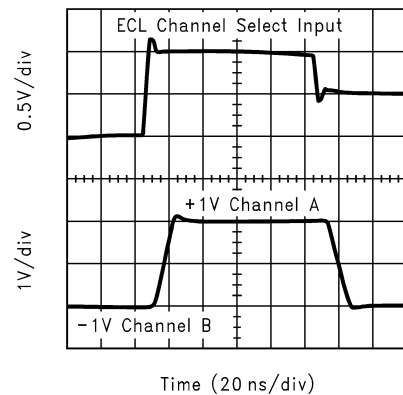
Large signal Channel-to-Channel Switching
