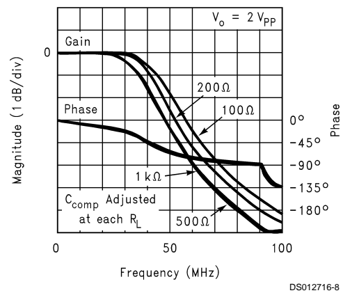
Large Signal Frequency Response vs. Load
