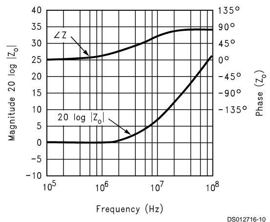
Output Impedance
