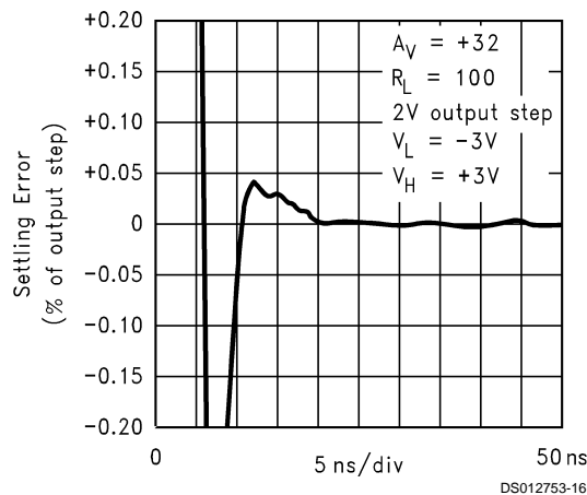
Settling, Unclamped
