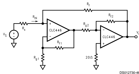
FIGURE 10. Composite Amplifier
