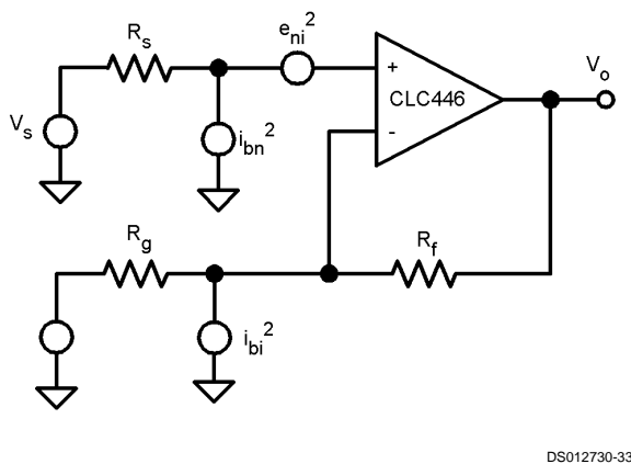
FIGURE 9. Noise Model
