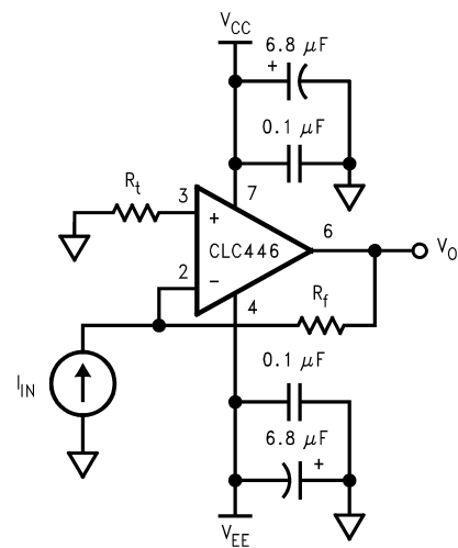
FIGURE 3. Transimpedance Gain
