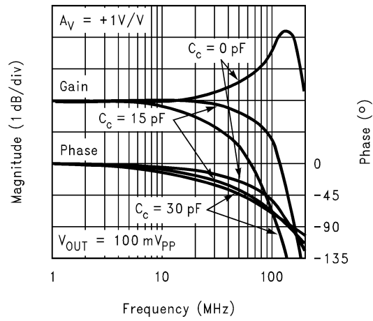
Frequency Response vs. Compensation Cap.
