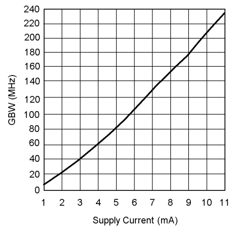
Gain-Bandwidth Product vs Supply Current
