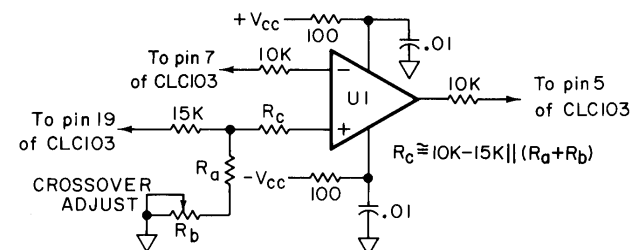
Figure 3: non-inverting gain composite amp to be used with figure 1 circuit
