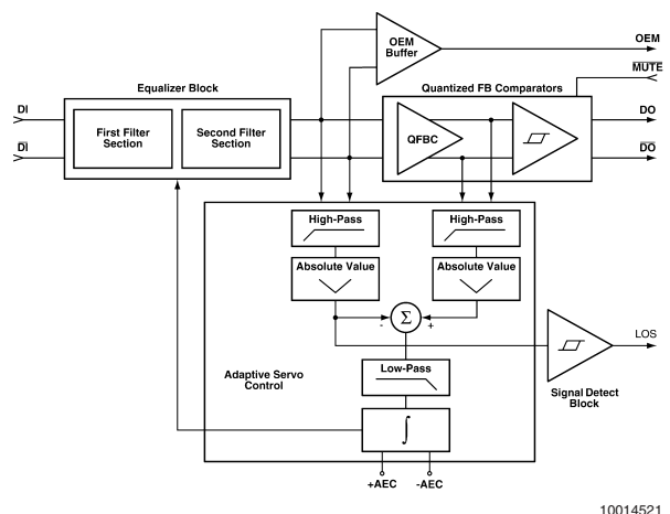
FIGURE 2. CLC012 Block Diagram
