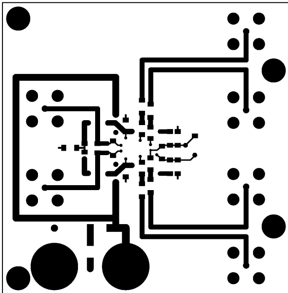
COMLINEAR LAYER2
