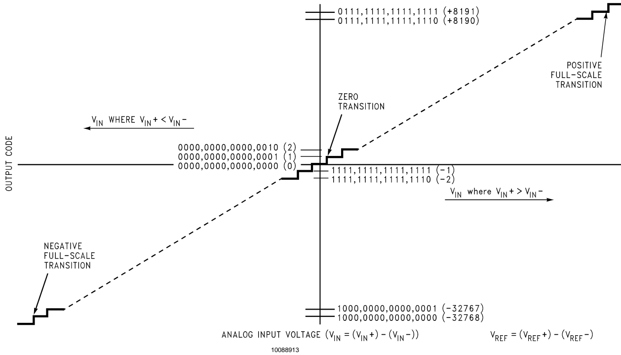
FIGURE 1. Transfer Characteristics
