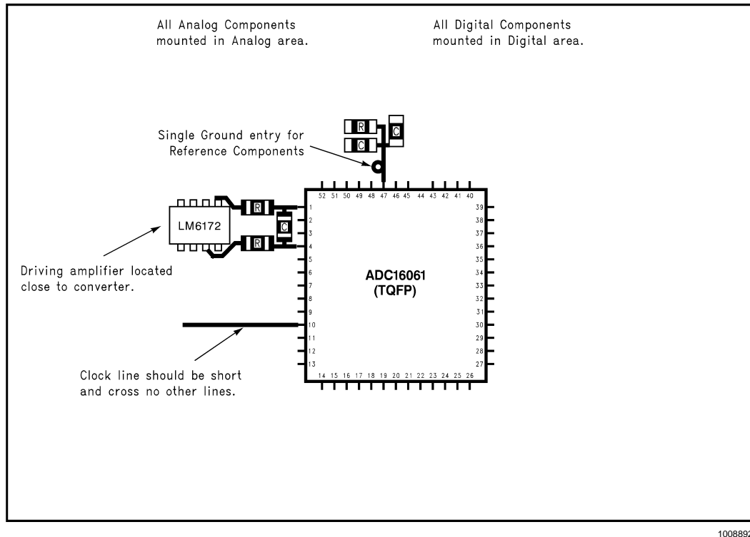
FIGURE 9. Example at a suitable layout.
