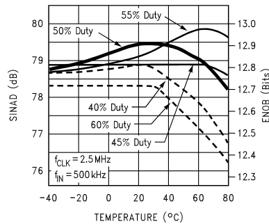
SINAD &amp; ENOB vs Clock Duty Cycle
