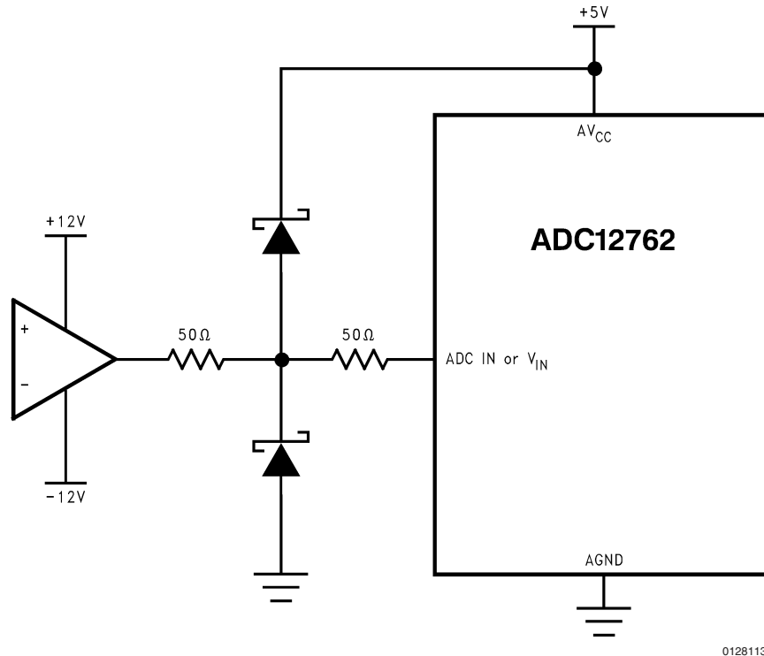
FIGURE 9. Input Protection
