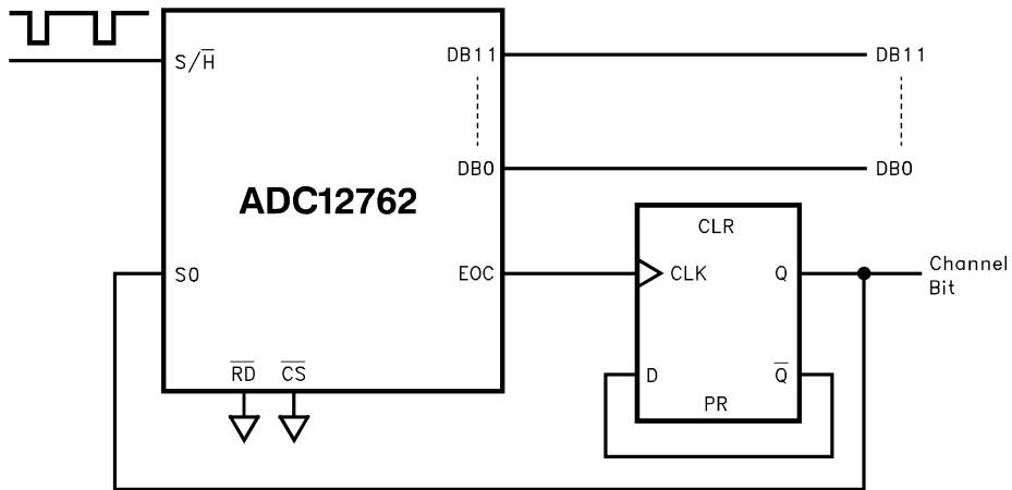
Ping-Pong between V_{IN1} and V_{IN2}
