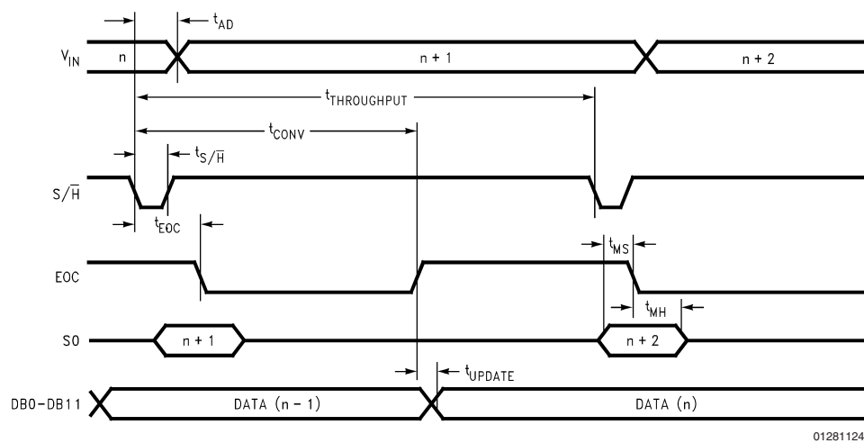
FIGURE 2. High Speed Interface Timing (MODE = 0, OE = 1, \overline{CS} = 0 , \overline{RD} = 0 )
