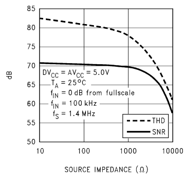
SNR and THD vs Source Impedance
