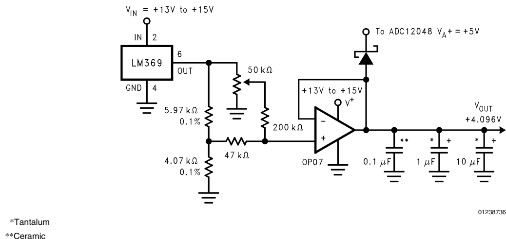
FIGURE 20. Low Drift Extremely Stable Reference Circuit
