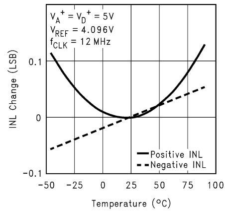
Integral Linearity Error (INL) Change vs. Temperature
