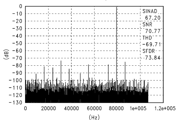
Full Scale Differential 79,468 Hz Sine Wave Input
