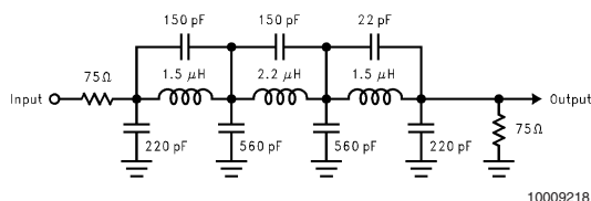
FIGURE 7. 5.5 MHz Low Pass Filter to Eliminate Harmonics at the Signal Input.
