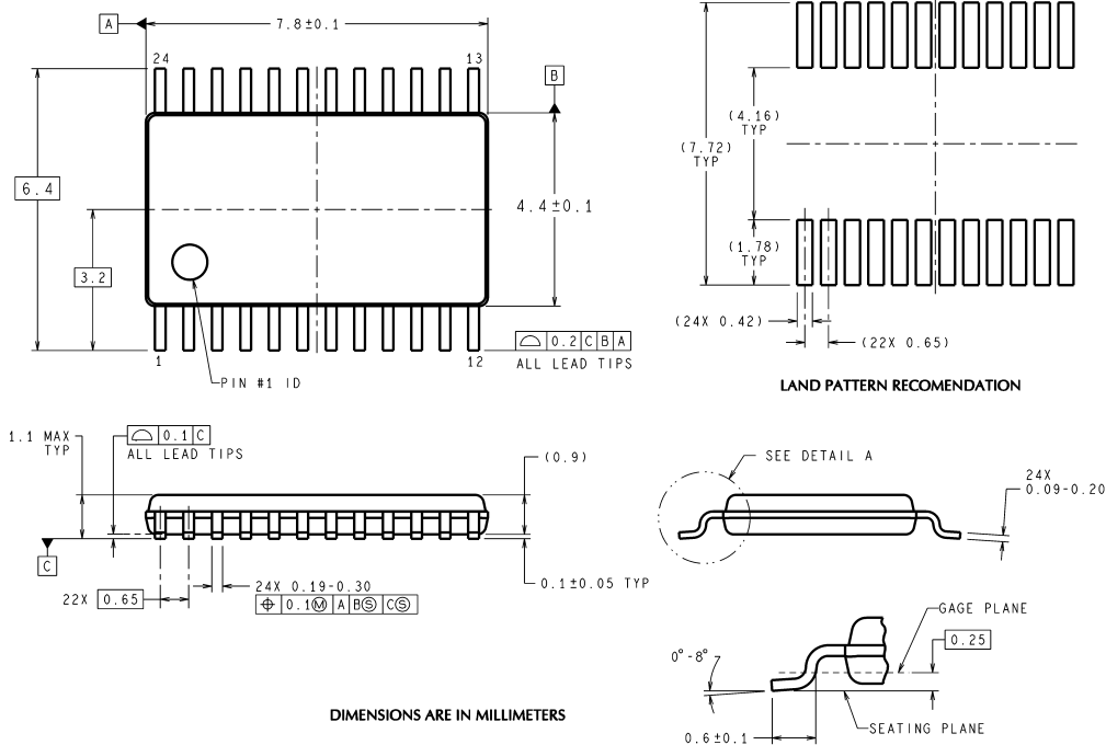
DETAIL A TYPICAL
