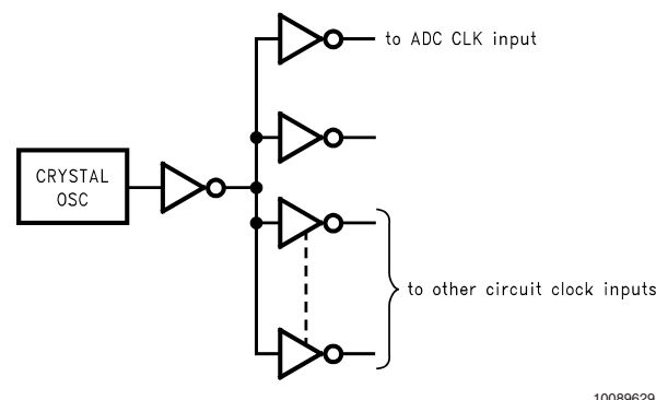
FIGURE 6. Isolating the ADC Clock from Digital Circuitry
