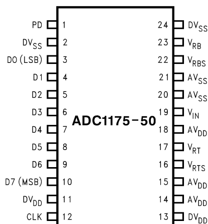
24-pin SOIC and TSSOP
